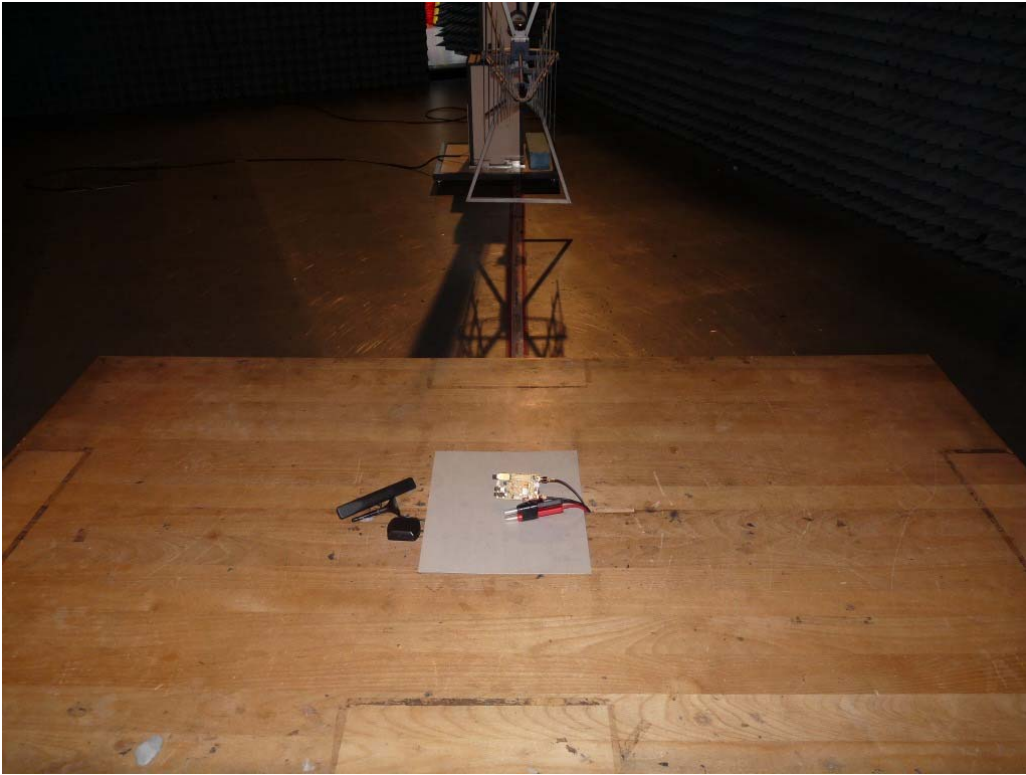
Photo 7: Test setup for radiated measurements (AC Port (power line), EUT supplied by external power supply, unintentional radiator §15)(RFID not active)
