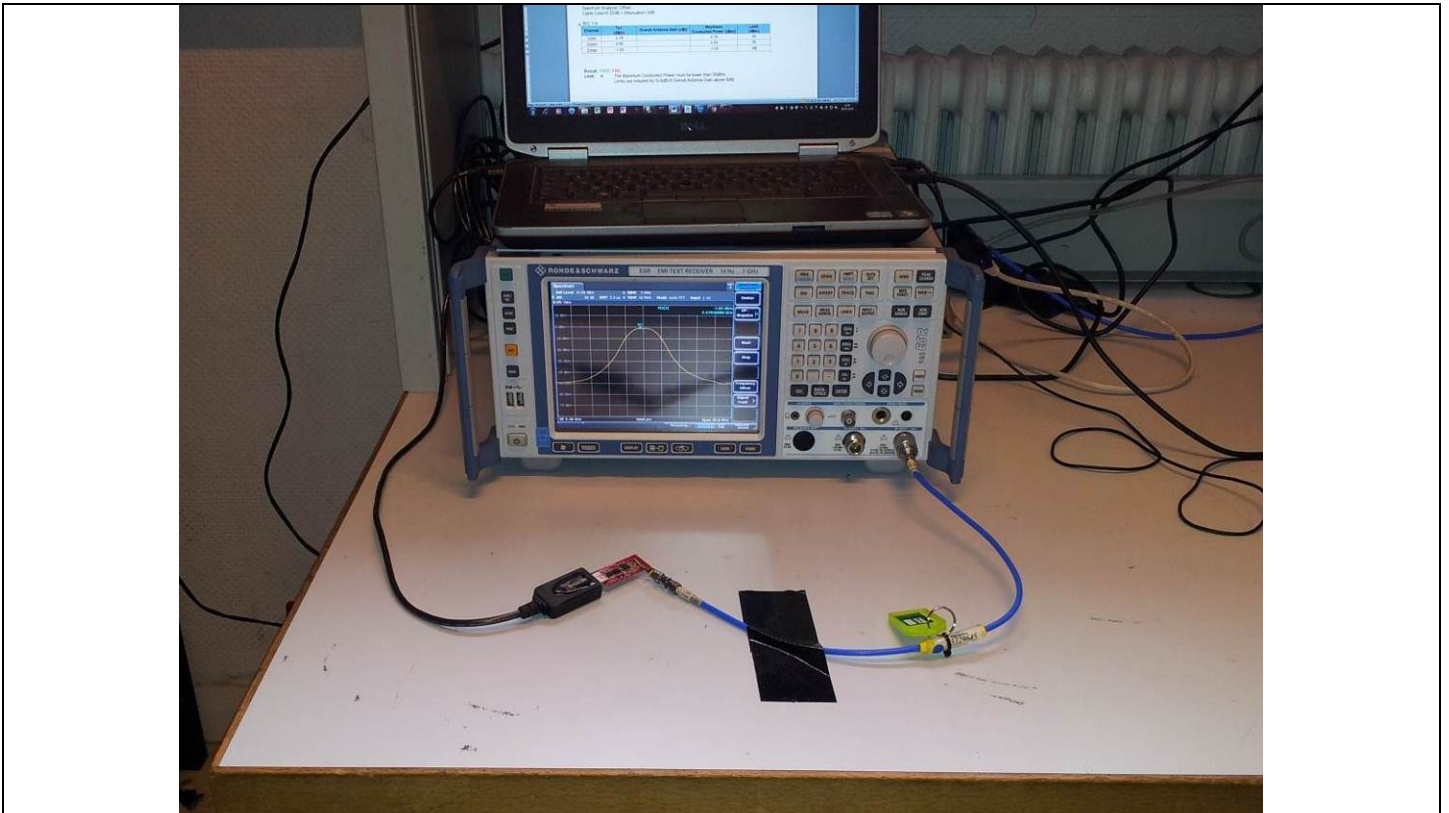
Photograph for Maximum Conducted Power
