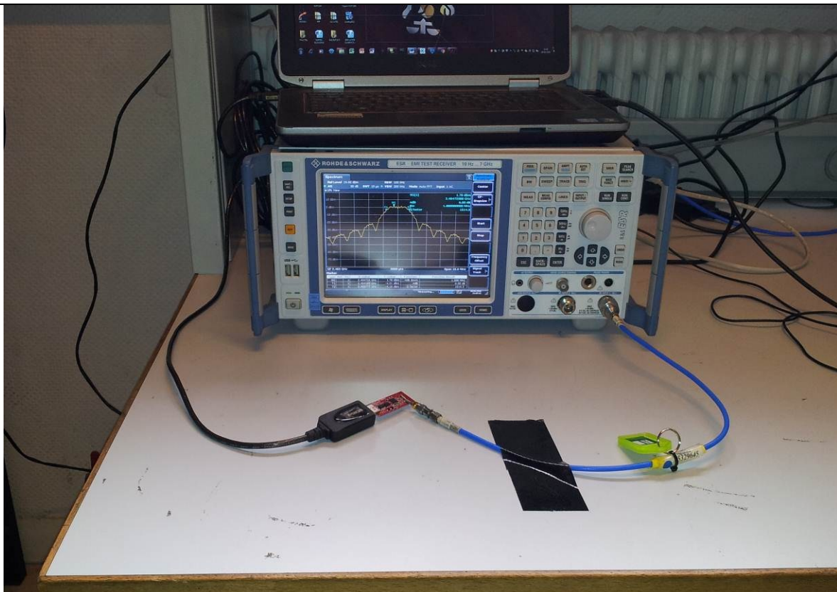
Photograph for -6dB Bandwidth
