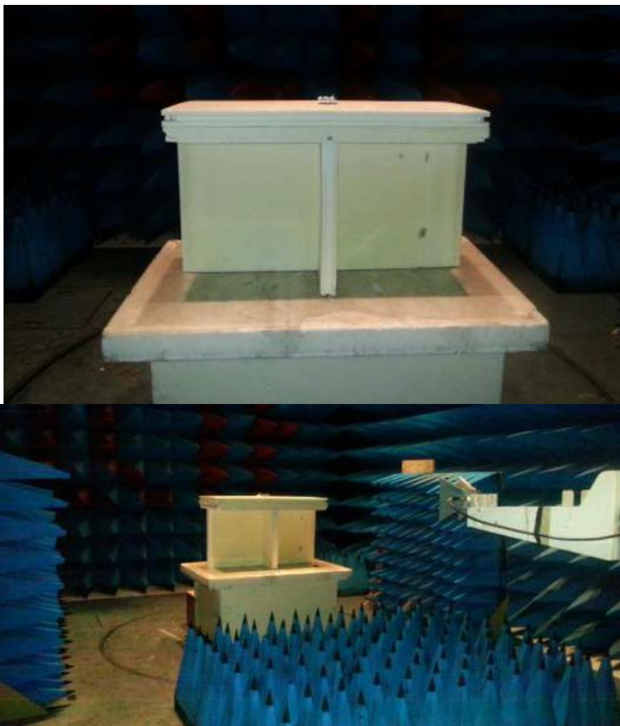
Radiated emissions measurements setup above 1GHz (JN5179-001-M10 version)
