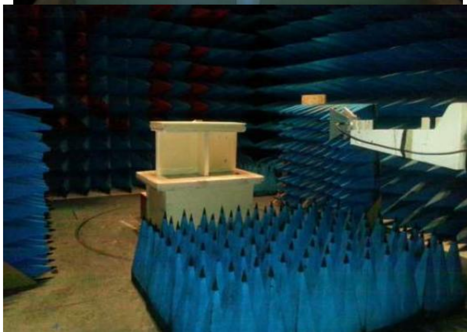
Radiated emissions measurements setup above 1GHz (JN5179-001-M13 version)
