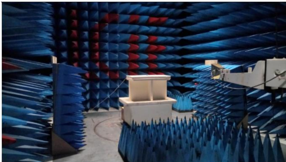
Radiated emissions measurements setup above 1GHz
