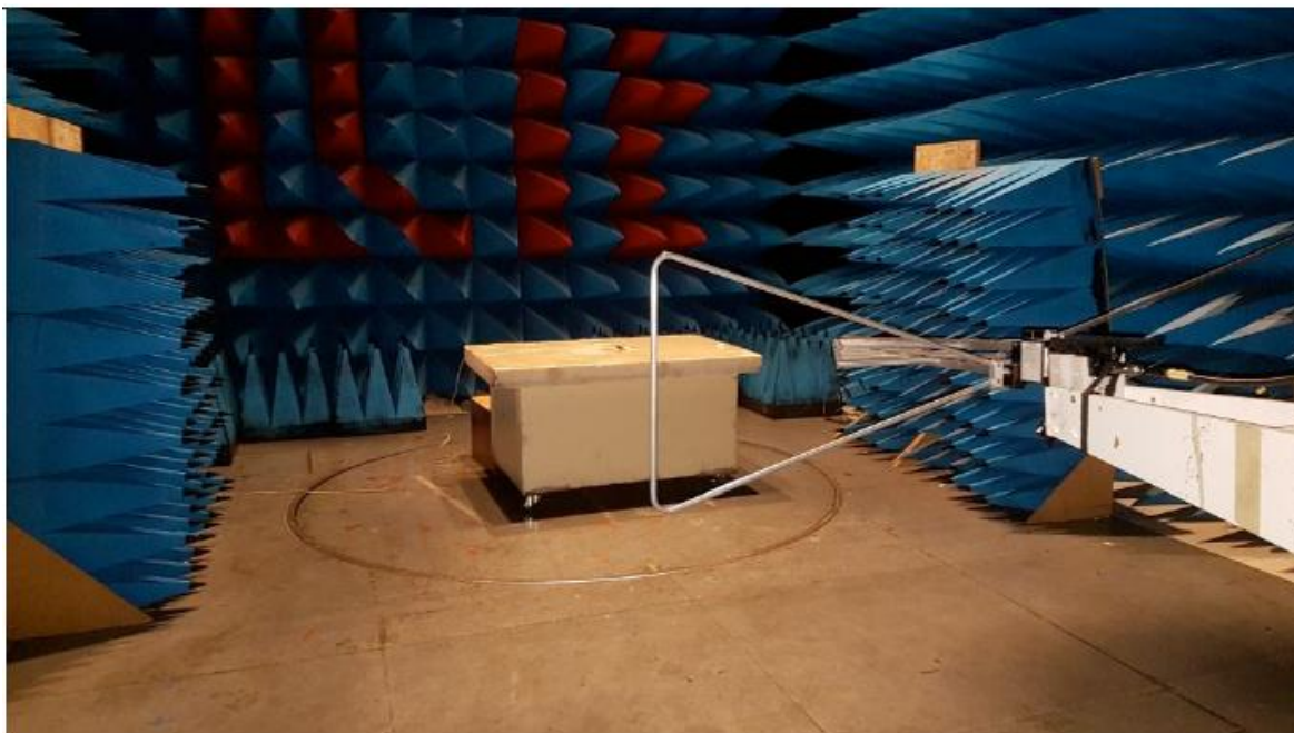
Radiated emissions measurements setup below 1GHz
