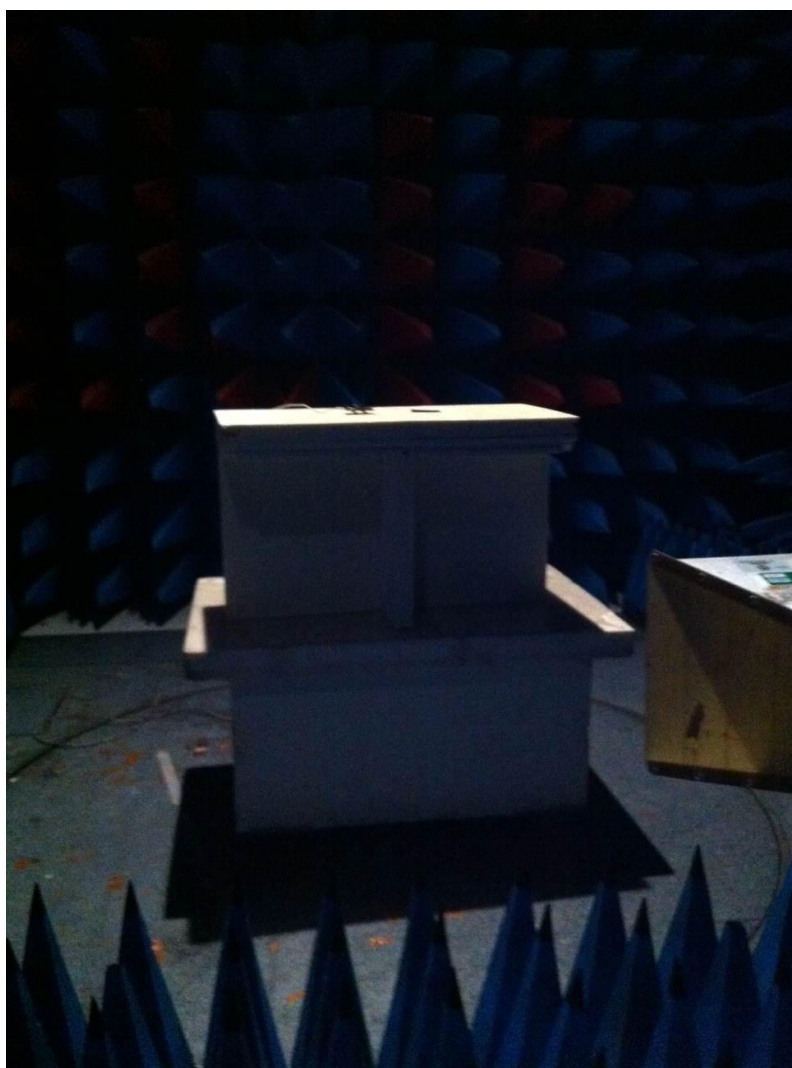
Radiated emissions measurements setup above 1GHz
