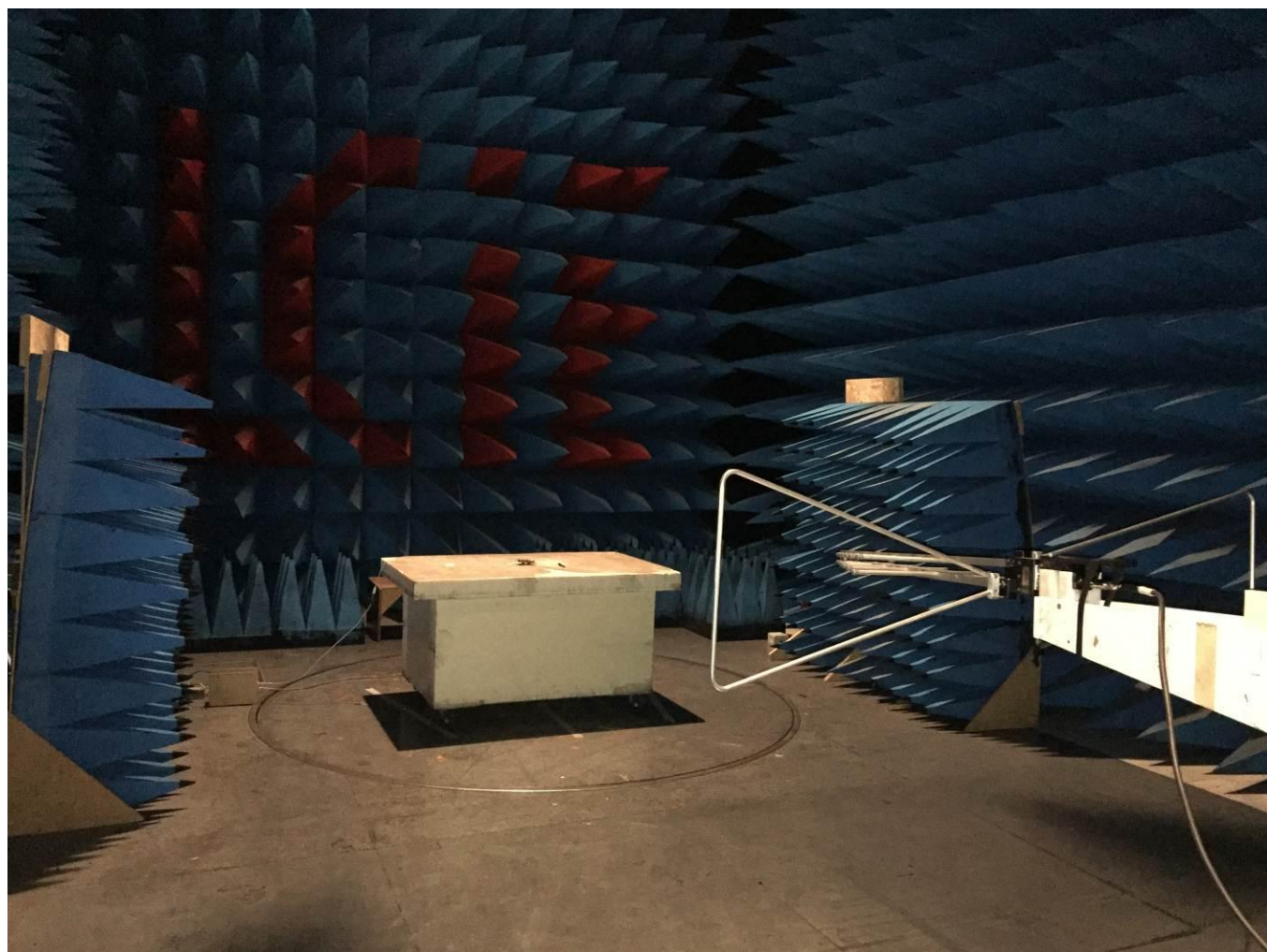
Radiated emissions measurements setup below 1GHz
