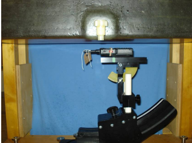
Face-Held Test Setup – STP9040, -00663 Antenna, -00635 Battery
