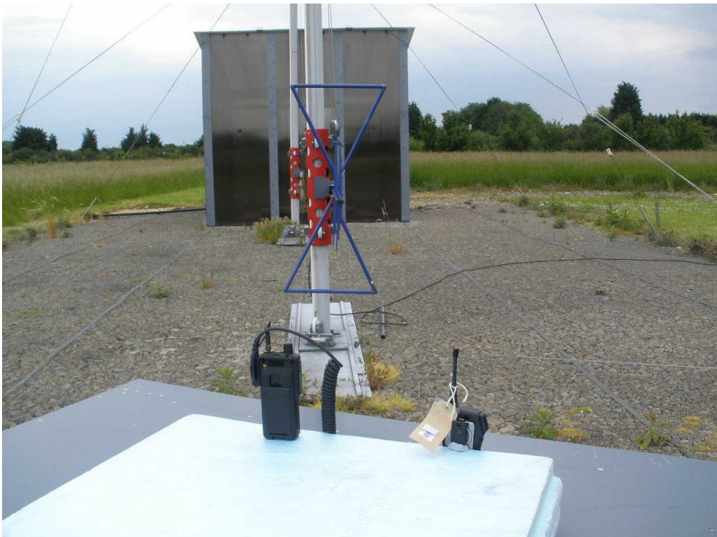
Photograph 5 With RSM: Radiated Emissions - Back
