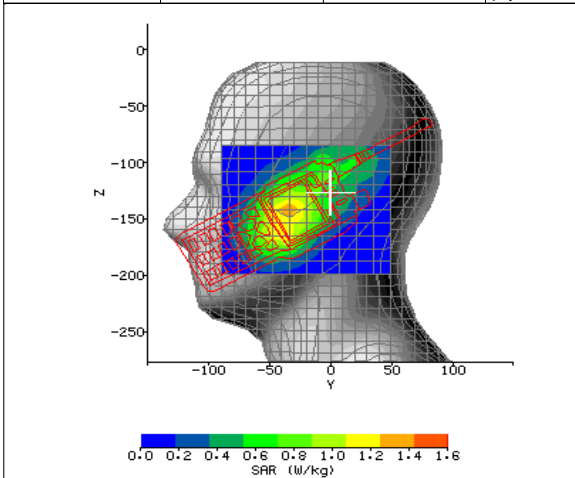
Figure 18: SAR Head Testing Results for the 8080 TETRA Portable at 854.025MHz.
