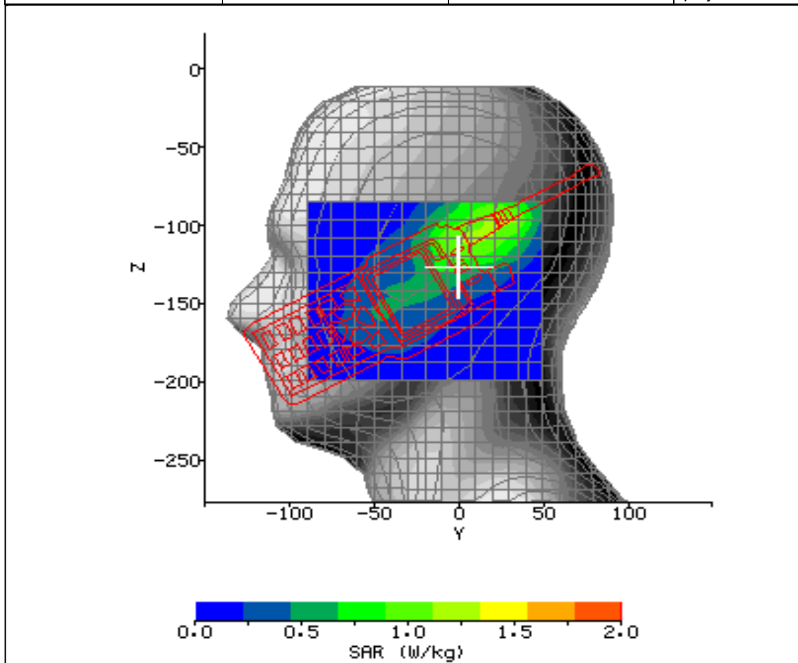
Figure 22: SAR Head Testing Results for the 8080 TETRA Portable at 854.025MHz. (Hi Capacity Battery)
