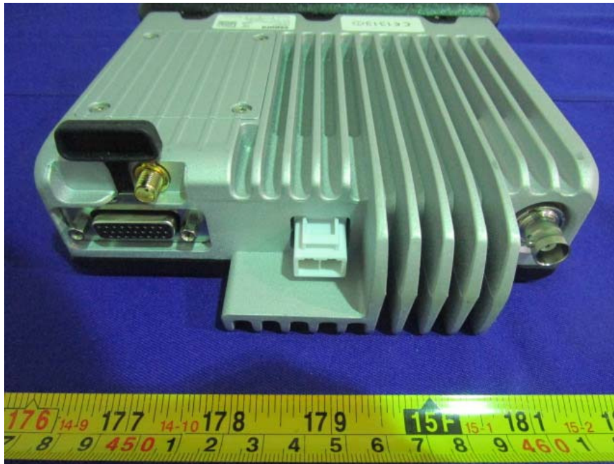
EUT-Rear View
