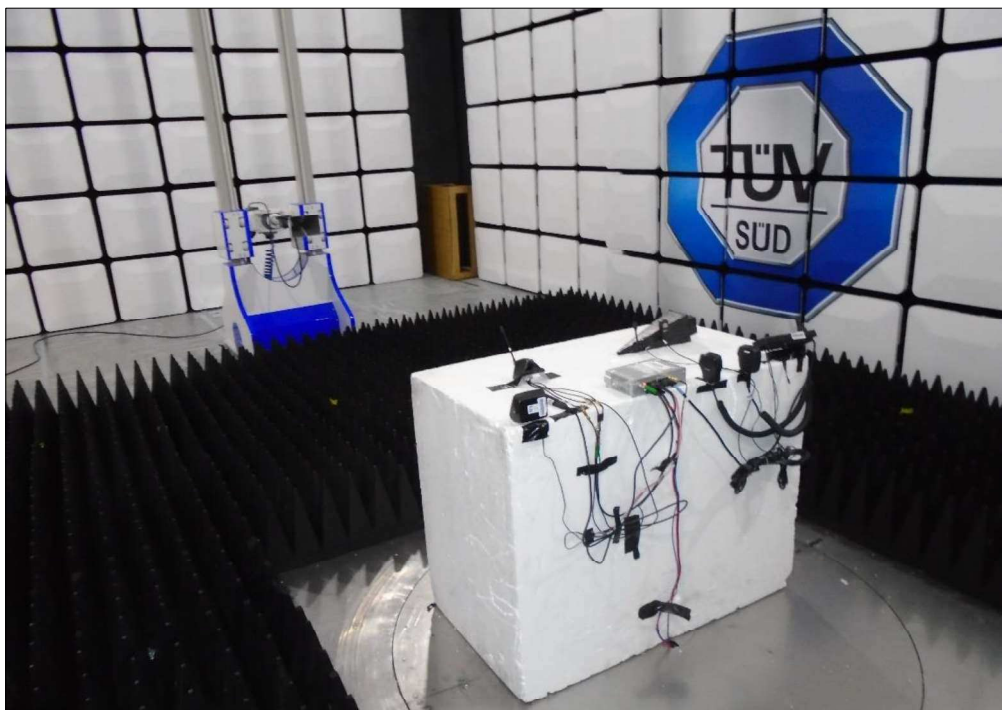
Figure 7 - Test Setup - Above 1 GHz
