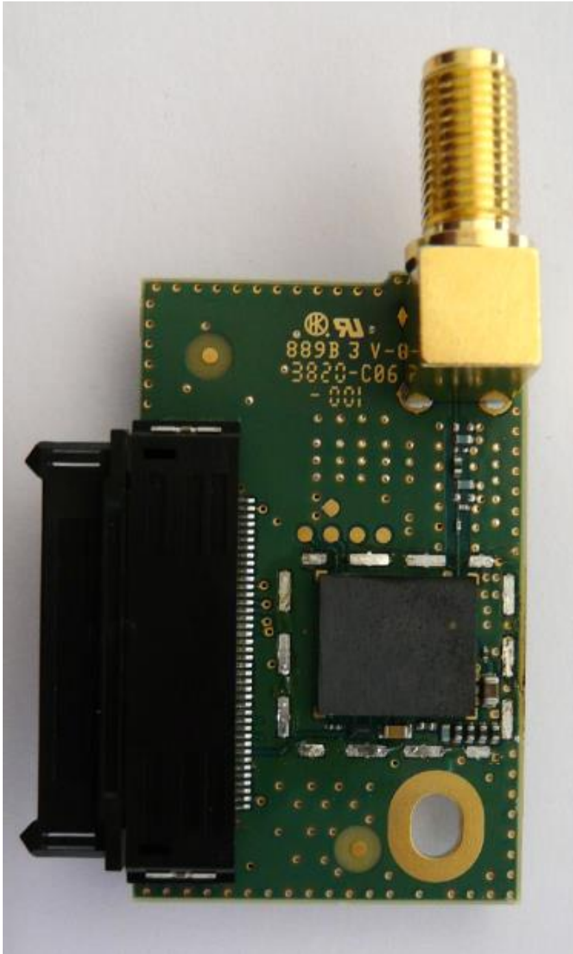
Figure 11. BT/Wi-Fi Board Top (Can Removed)
