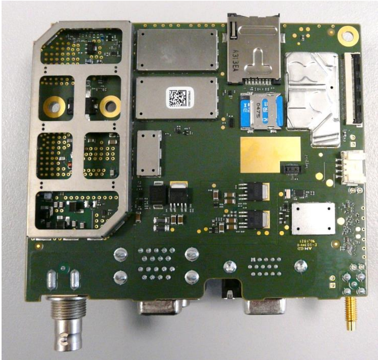
Figure 1. Main Board Bottom
