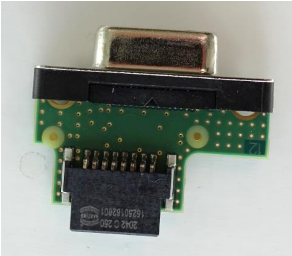
Figure 8. FC2 RC4 Board Top
