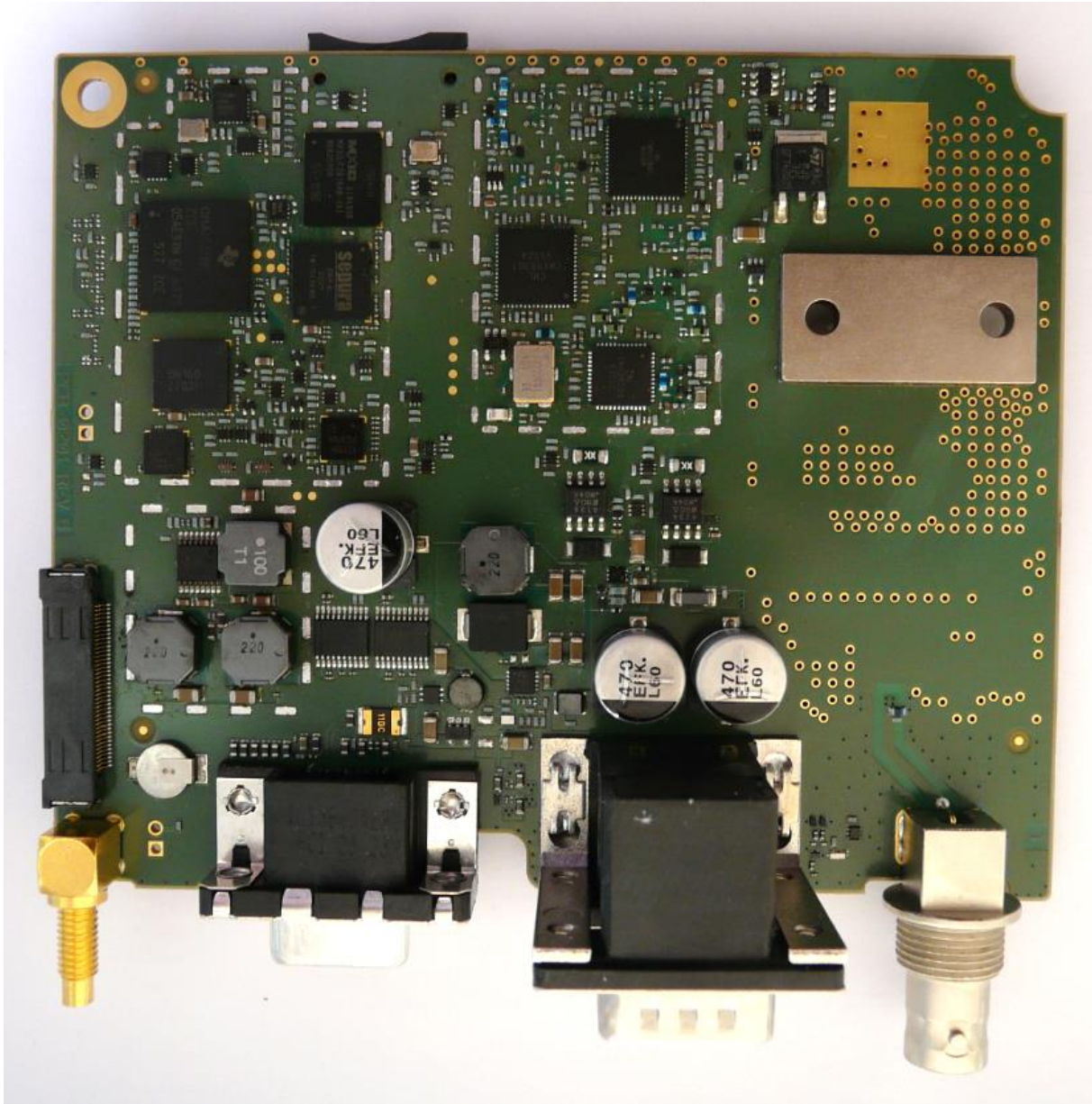
Figure 4. Main Board Top cans removed
