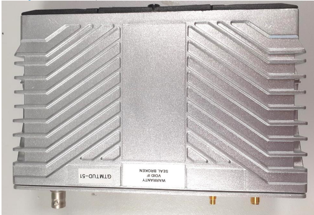
Figure 9. Top View
