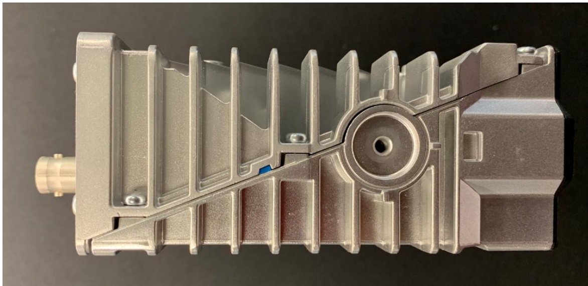
Figure 7. Side View 2
