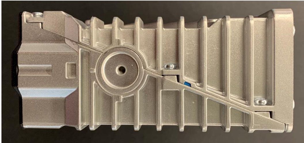
Figure 6. Side View 1
