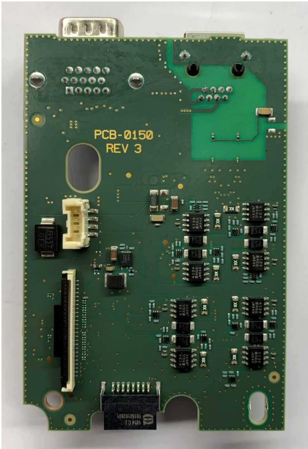
Figure 7. SCG2229 / XX6SCG2229W / 8739A-SCG2229 Expansion Board Bottom
