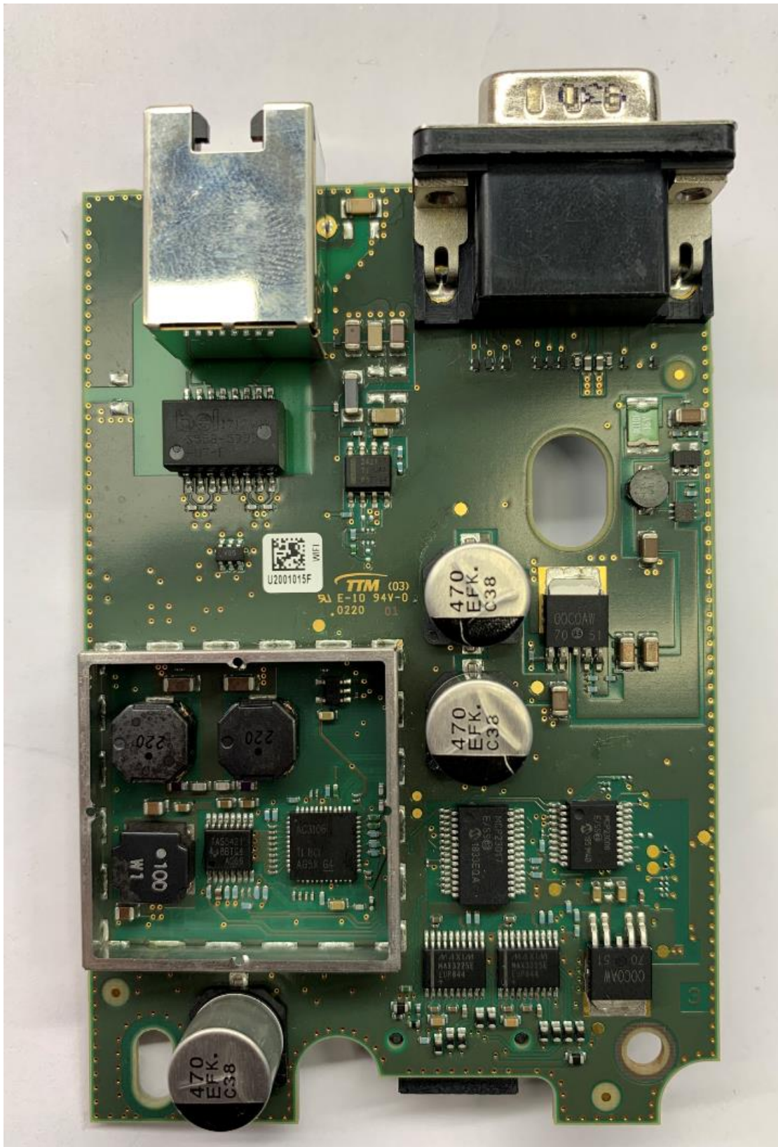
Figure 6. SCG2229 / XX6SCG2229W / 8739A-SCG2229 Expansion Board Top (Can Removed)
