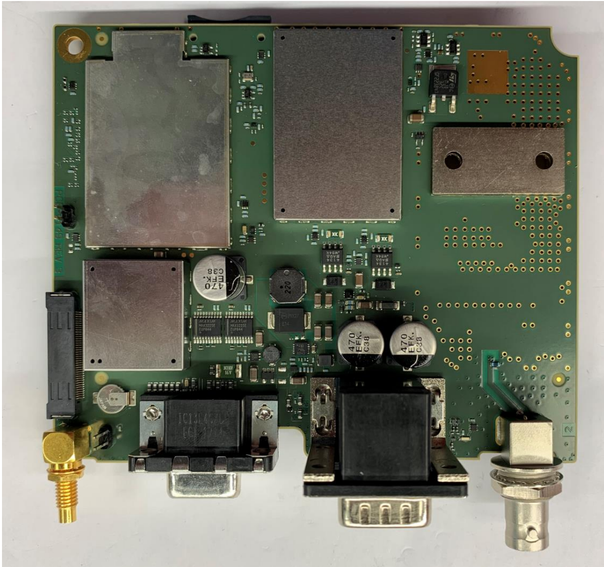
Figure 3. SCG2229 / XX6SCG2229W / 8739A-SCG2229 Main Board Top
