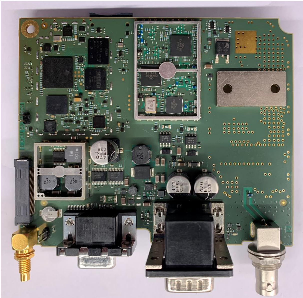
Figure 4. SCG2229 / XX6SCG2229W / 8739A-SCG2229 Main Board Top cans removed
