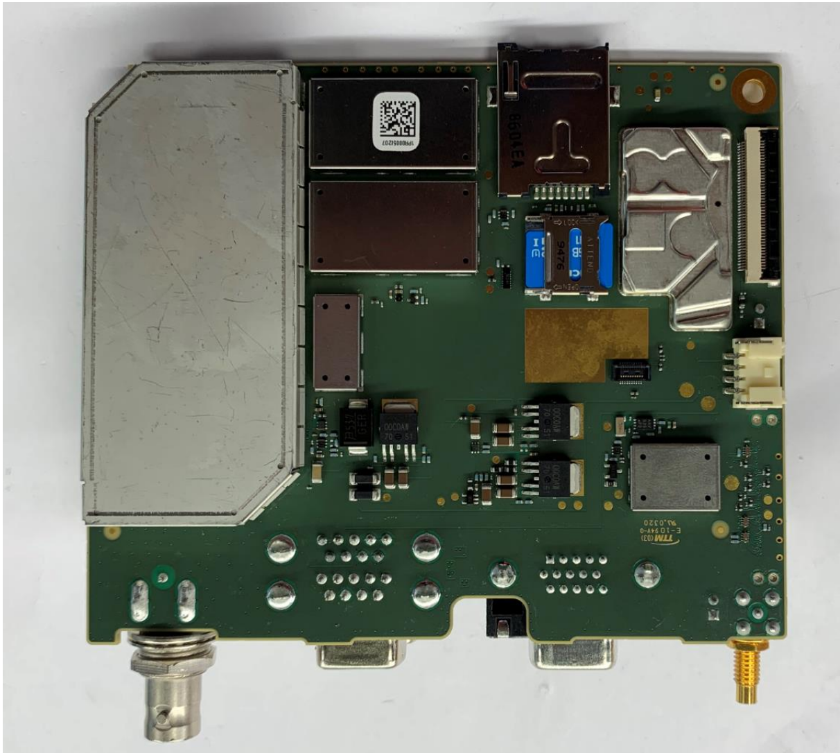
Figure 1. SCG2229 / XX6SCG2229W / 8739A-SCG2229 Main Board Bottom
