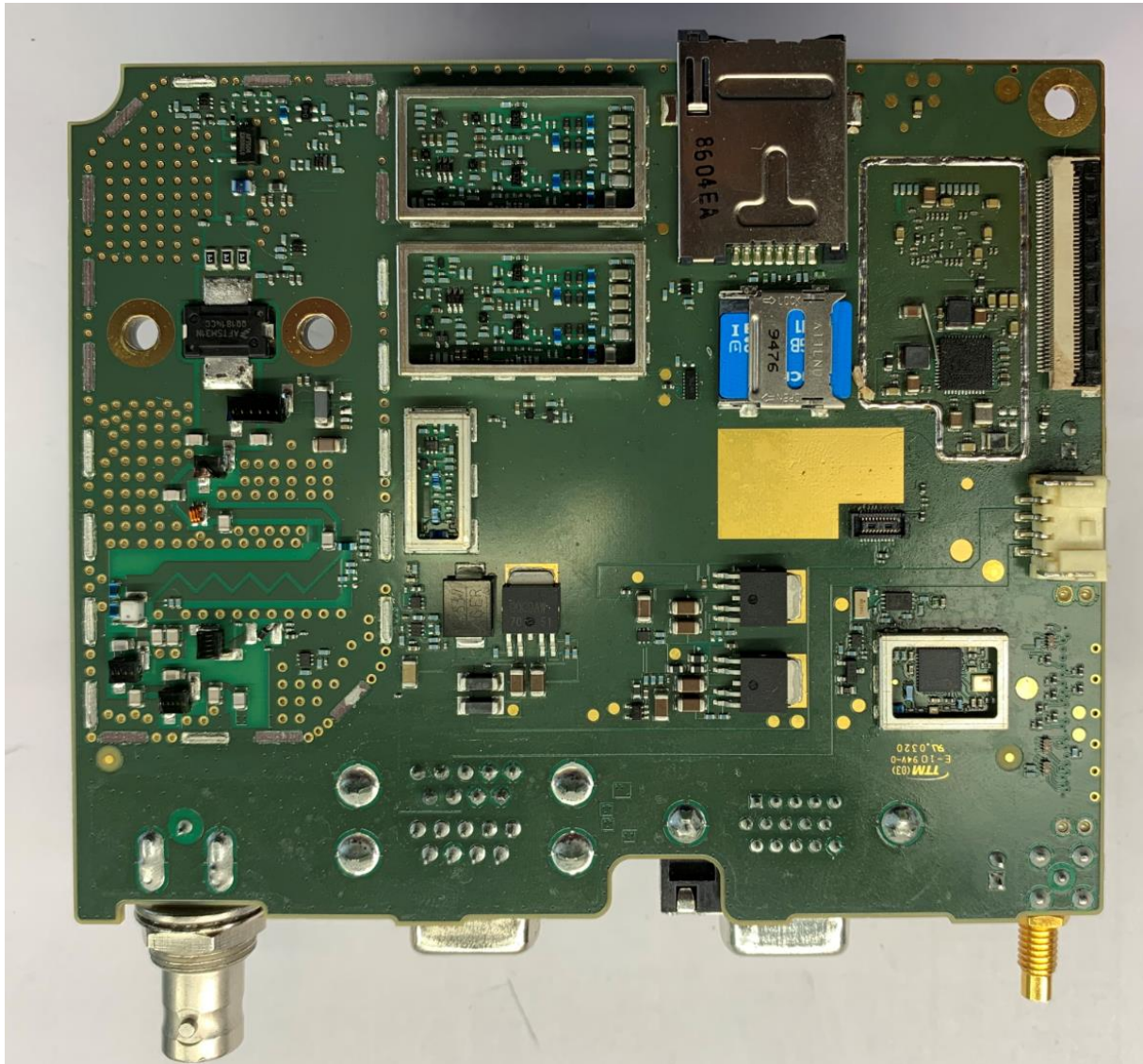
Figure 2. SCG2229 / XX6SCG2229W / 8739A-SCG2229 Main Board Bottom with cans removed
