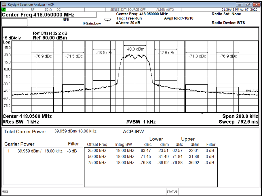
Figure 76 - 418.0500 MHz
