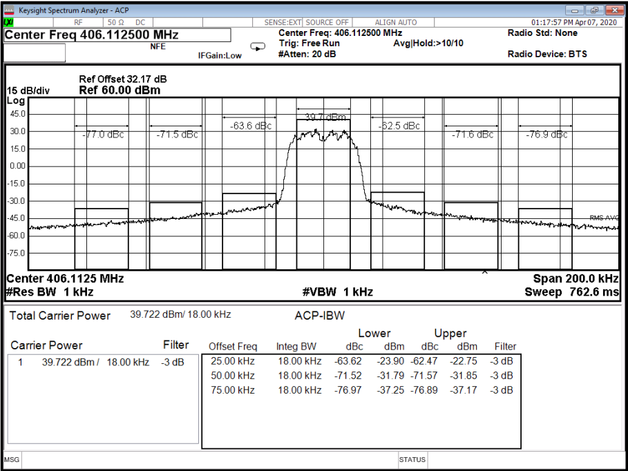
Figure 75 - 406.1125 MHz
