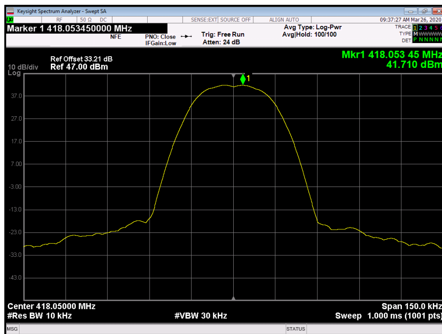
Figure 4 - Frequency Spectrum
