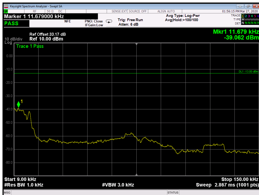
Figure 17 - 406.1125 MHz, 9 kHz to 150 kHz
