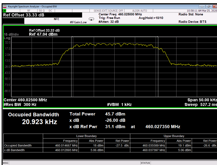
Figure 12 - 460.025 MHz
