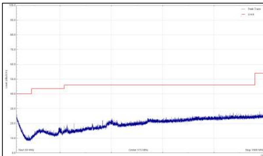
Figure 80 - 2437 MHz (CH6), 802.11n 20 MHz, 30 MHz to 1 GHz, Horizontal (Peak)
