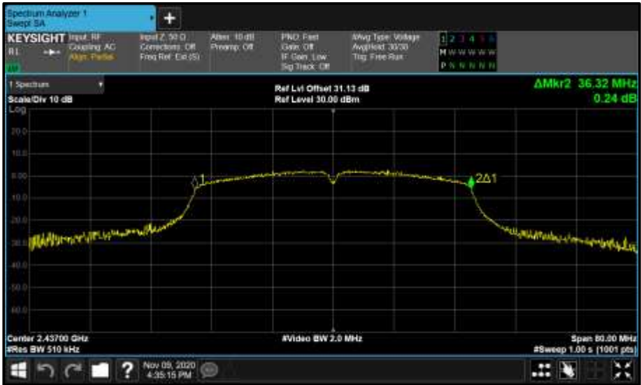
Figure 29 - (A) 2437 MHz (CH6) 99% Bandwidth
