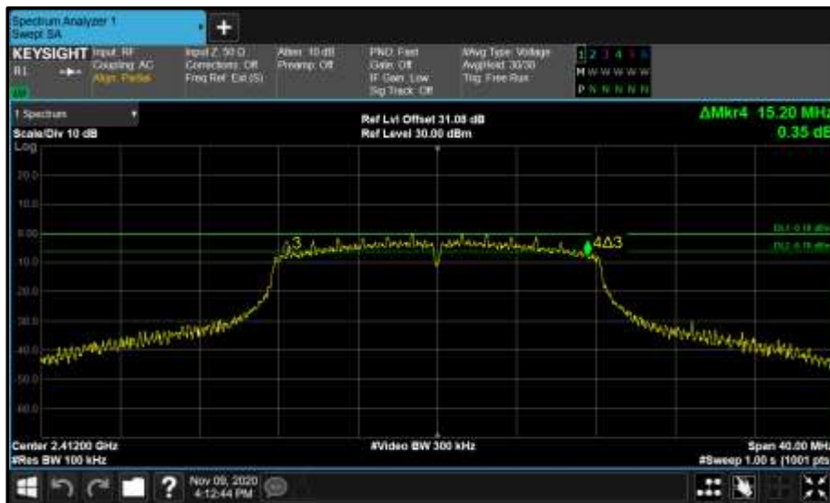
Figure 16 - (A) 2412 MHz (CH1) 6 dB Bandwidth
