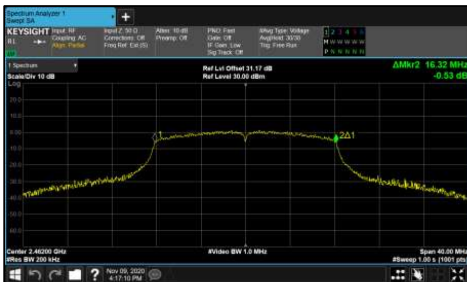
Figure 19 - (A) 2462 MHz (CH11) 99% Bandwidth
