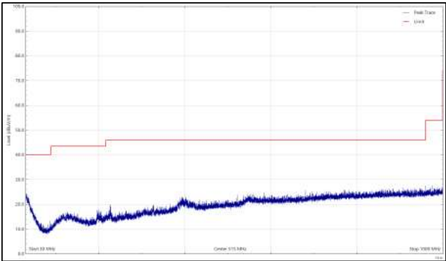
Figure 68 - 2462 MHz (CH11), 802.11g, 30 MHz to 1 GHz, Horizontal (Peak)
