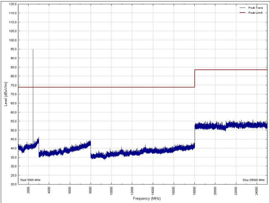
Figure 21 - 2440 MHz - 1 GHz to 25 GHz, Horizontal, EUT Orientation: X, Peak
