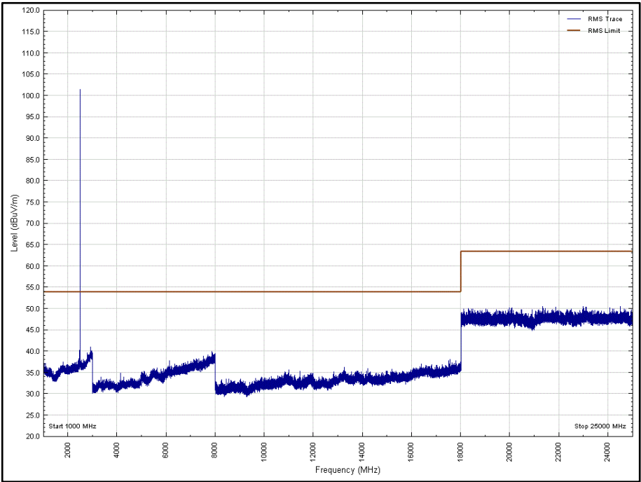
Figure 26 - 2480 MHz – 1 GHz to 25 GHz, Vertical, X Orientation - Average
