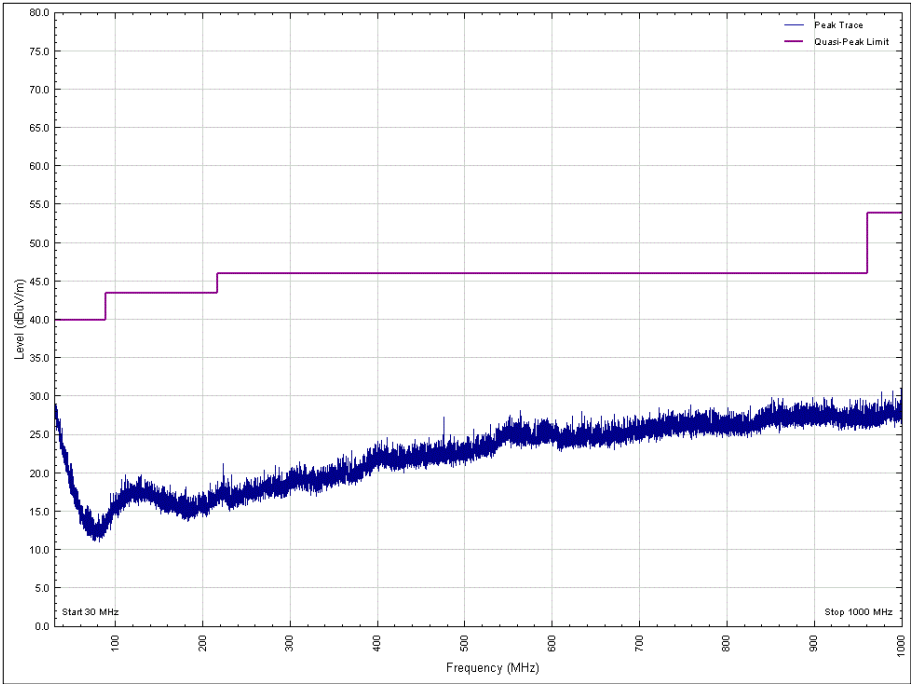
Figure 18 - 2440 MHz, 30 MHz to 1 GHz, Horizontal, X Orientation
