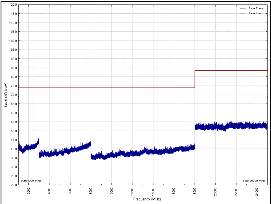
Figure 27 - 2480 MHz – 1 GHz to 25 GHz, Horizontal, X Orientation - Peak
