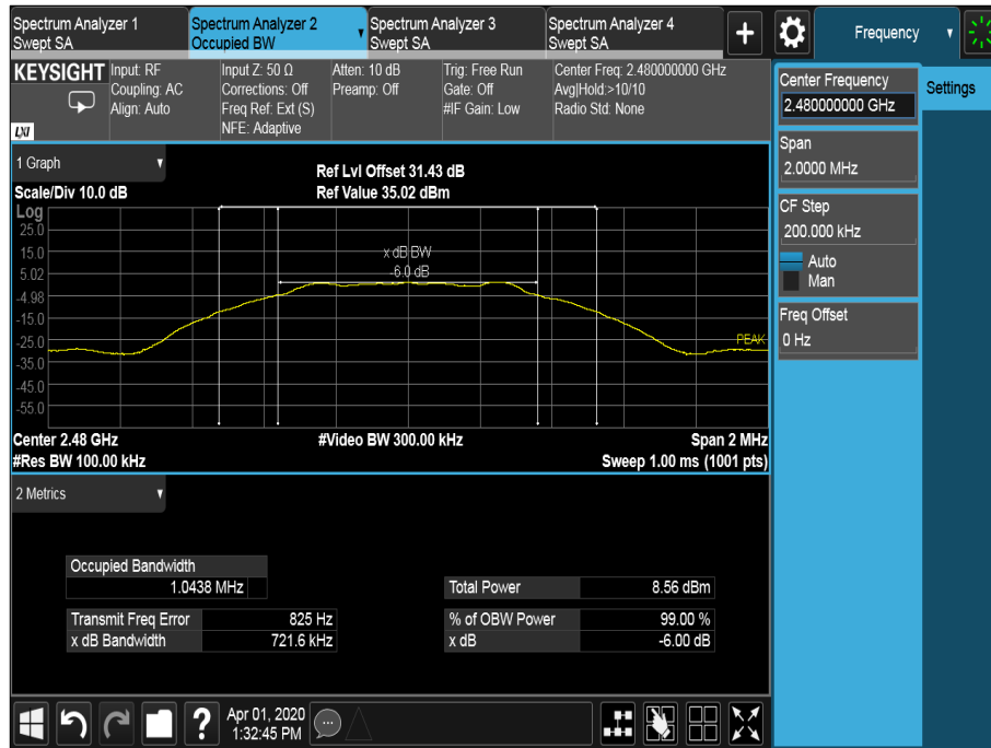
Figure 6 - 2480 MHz
