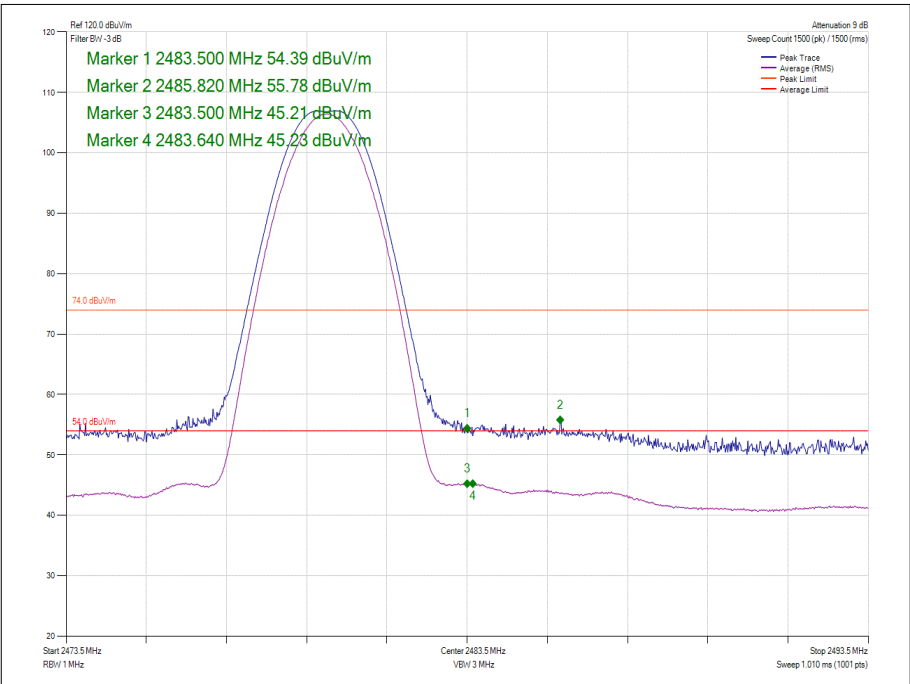
Figure 9 - GFSK - 2480 MHz - Band Edge Frequency 2483.5 MHz
