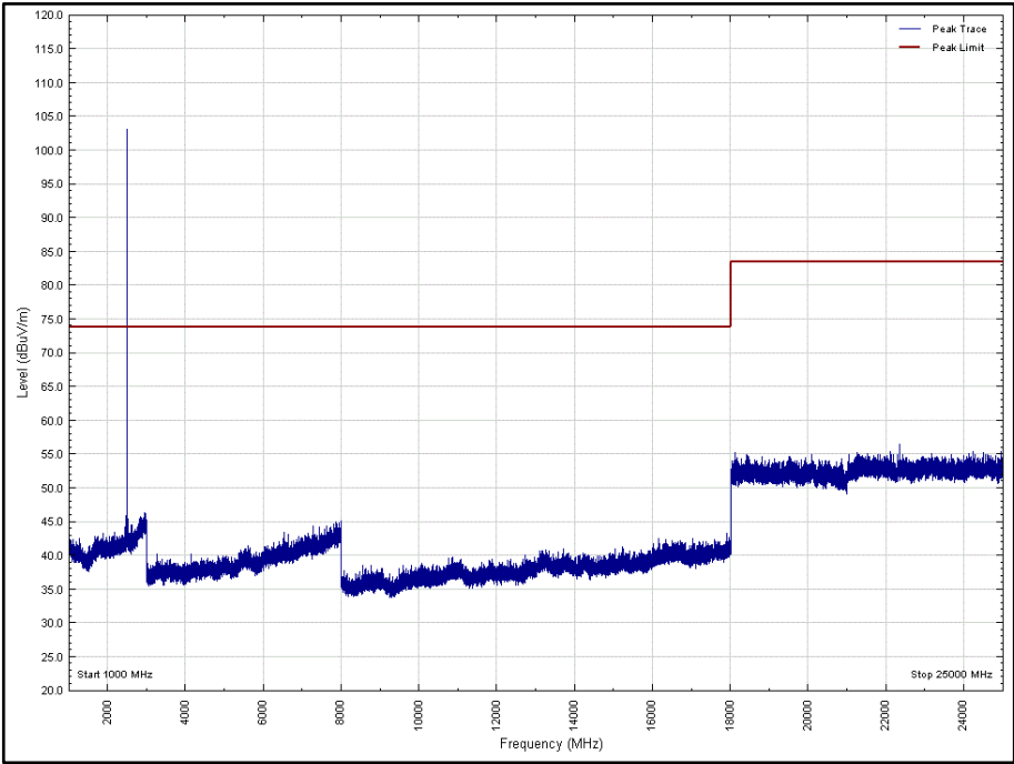
Figure 25 - 2480 MHz – 1 GHz to 25 GHz, Vertical, X Orientation – Peak
