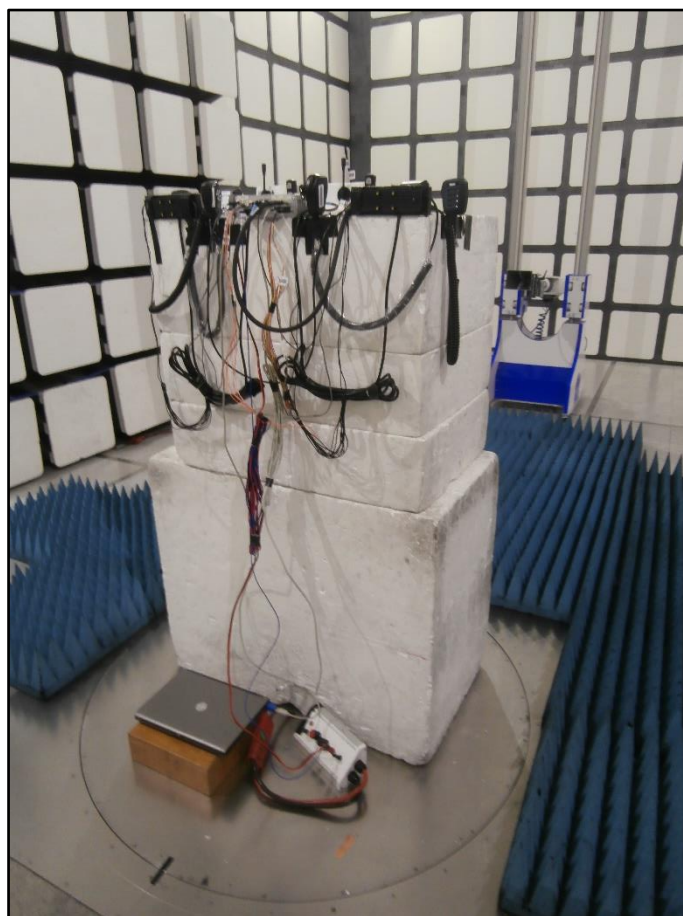
Figure 30 - Test Setup – 1 GHz to 8 GHz – X Orientation
