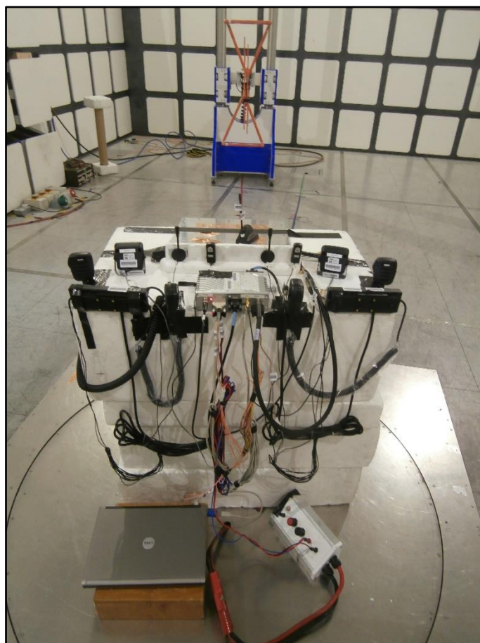
Figure 29 - Test Setup – 30 MHz to 1 GHz – X Orientation
