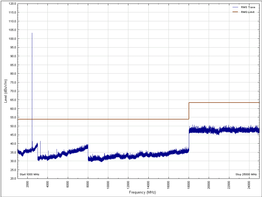
Figure 20 - 2440 MHz - 1 GHz to 25 GHz, Vertical, X Orientation - Average
