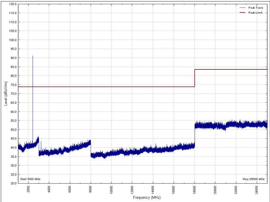
Figure 15 - 2402 MHz, 1 GHz to 25 GHz, Horizontal, X Orientation - Peak
