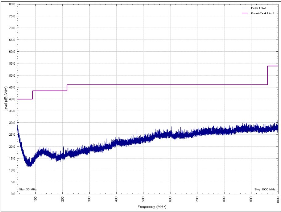
Figure 17 - 2440 MHz, 30 MHz to 1 GHz, Vertical, X Orientation
