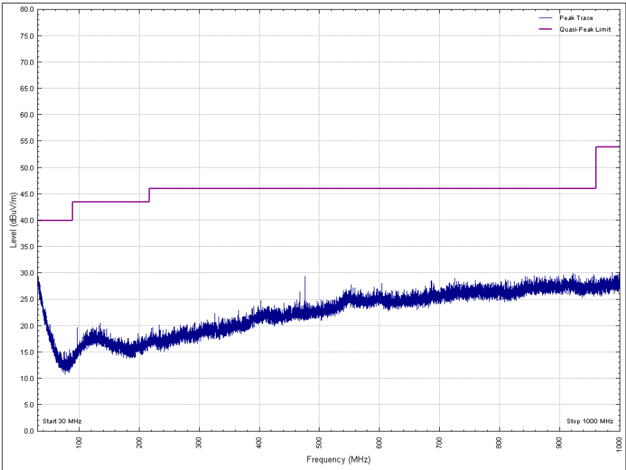
Figure 12 - 2402 MHz, 30 MHz to 1 GHz, Horizontal, X Orientation
