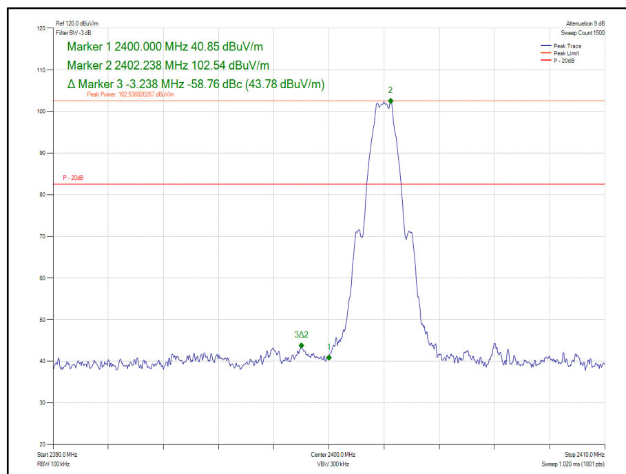
Figure 7 – GFSK, 2402 MHz - Measured Frequency 2400 MHz
