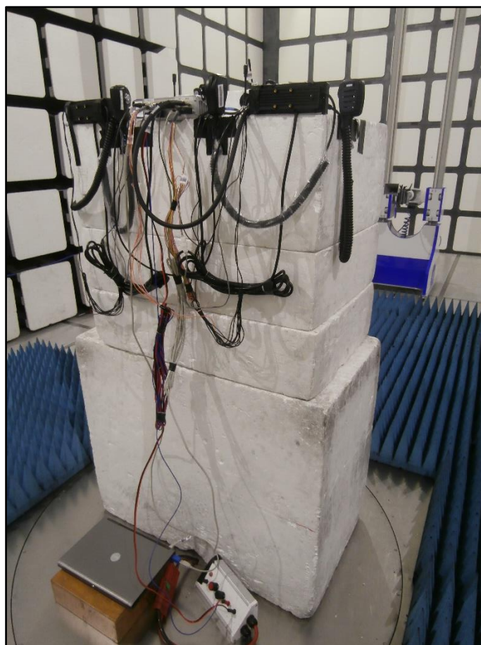
Figure 31 - Test Setup – 8 GHz to 18 GHz – X Orientation
