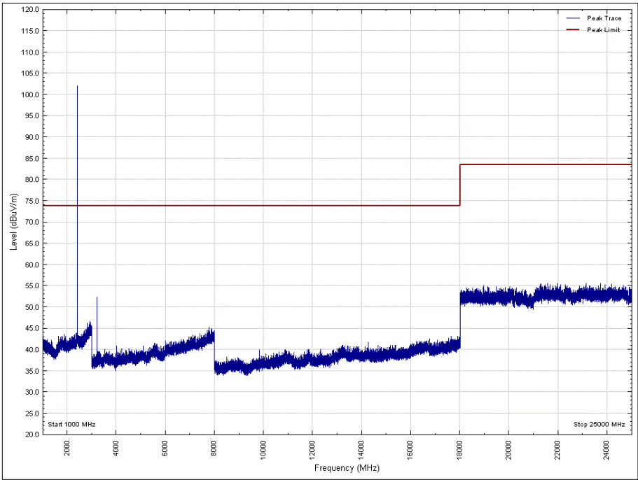
Figure 13 - 2402 MHz, 1 GHz to 25 GHz, Vertical, X Orientation - Peak
