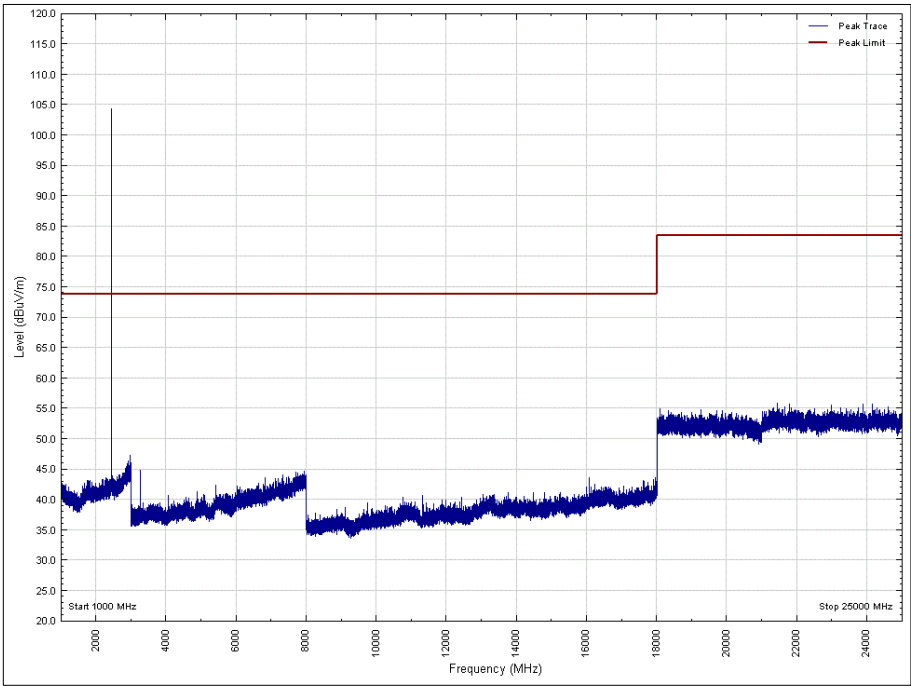
Figure 19 - 2440 MHz - 1 GHz to 25 GHz, Vertical, X Orientation X - Peak
