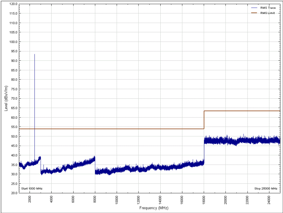
Figure 22 - 2440 MHz - 1 GHz to 25 GHz, Horizontal, X Orientation - Average
