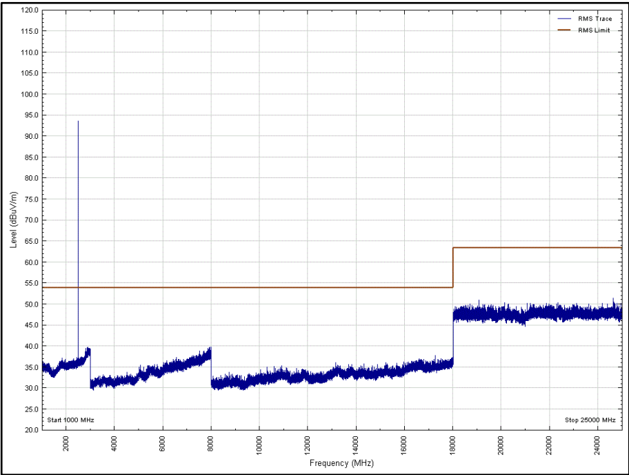
Figure 28 - 2480 MHz – 1 GHz to 25 GHz, Horizontal, X Orientation - Average
