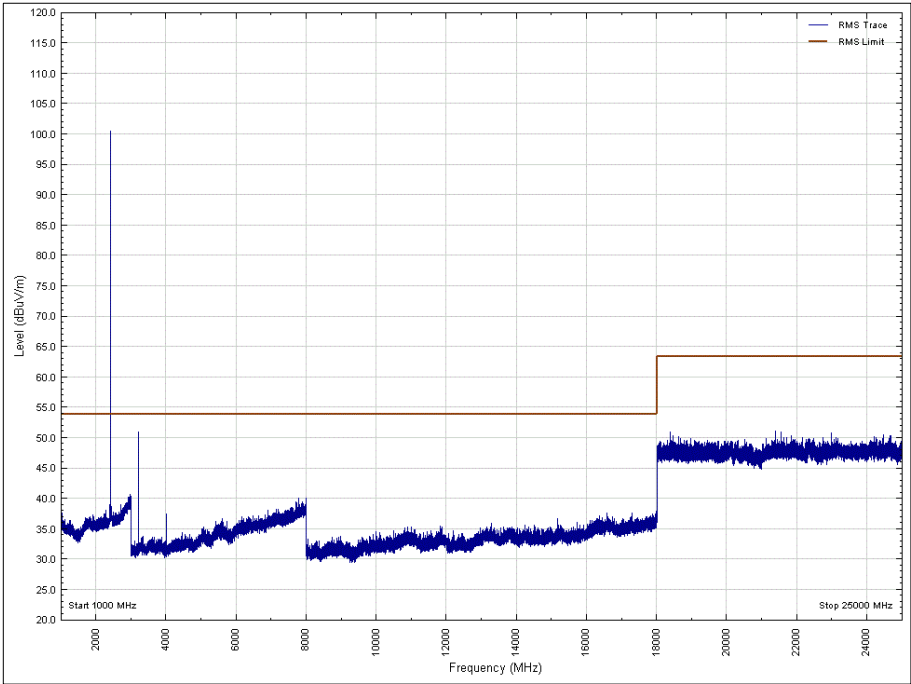
Figure 14 - 2402 MHz, 1 GHz to 25 GHz, Vertical, X Orientation - Average
