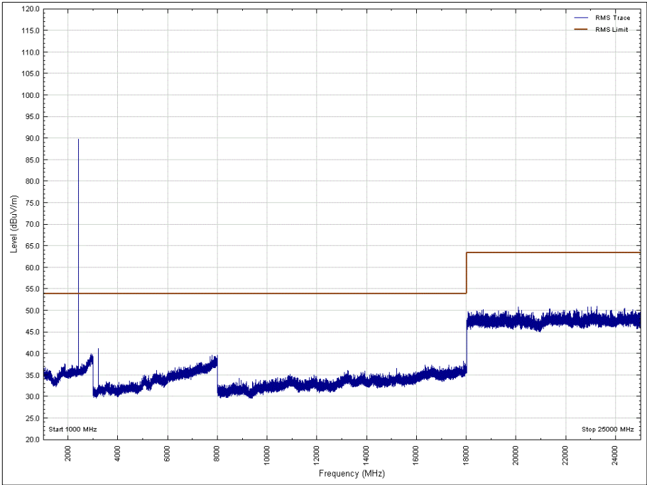
Figure 16 - 2402 MHz, 1 GHz to 25 GHz, Horizontal, X Orientation - Average
