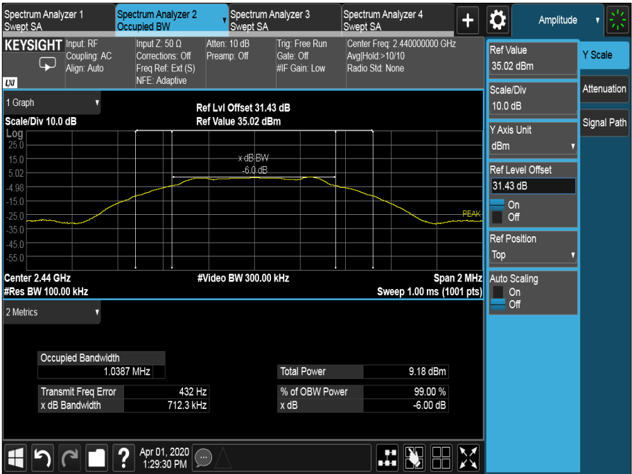
Figure 5 - 2440 MHz
