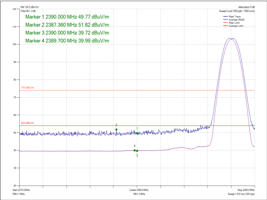
Figure 8 - GFSK - 2402 MHz - Band Edge Frequency 2390.0 MHz
