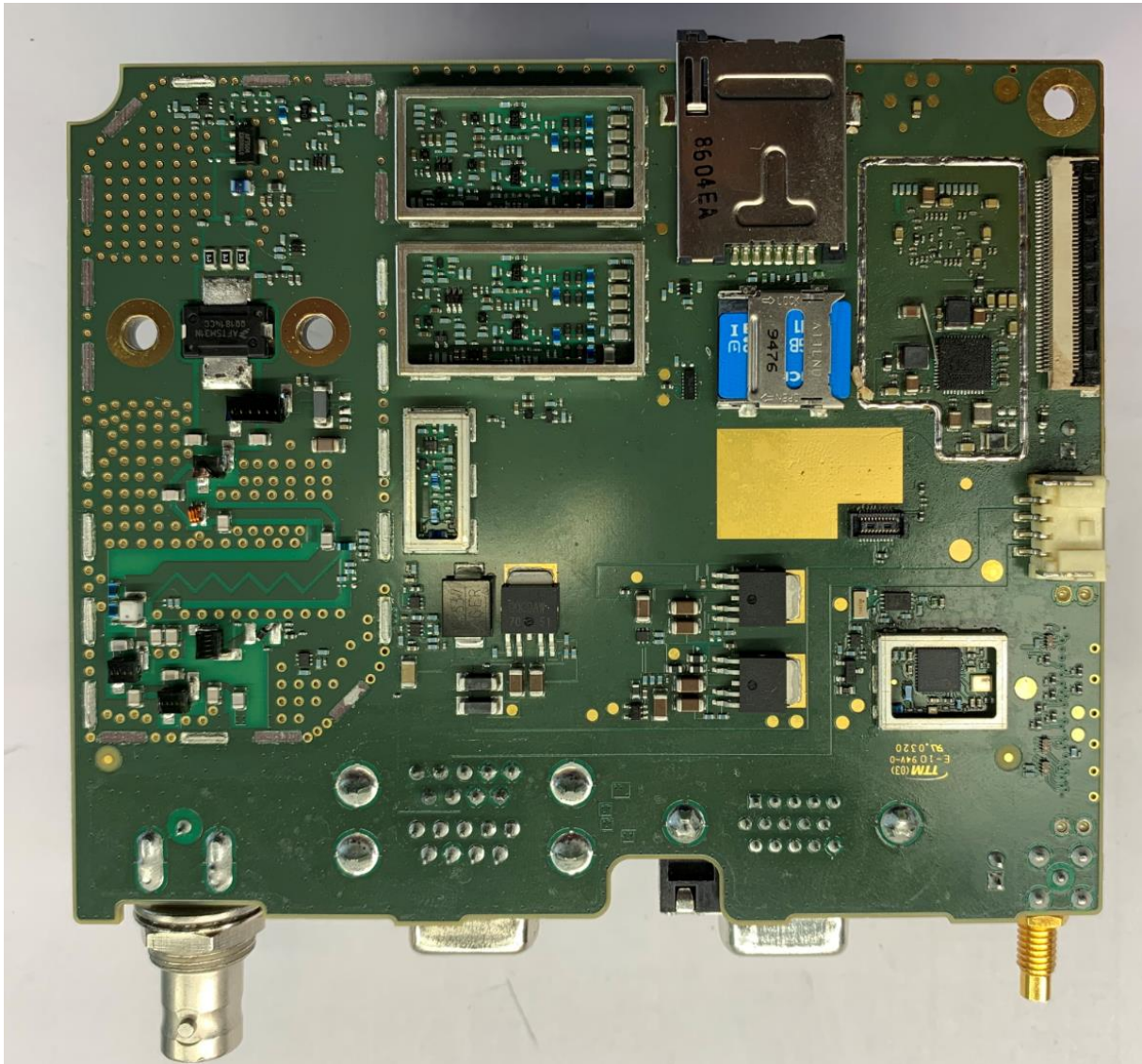
Figure 2. SCG2229 / XX6SCG2229 / 8739A-SCG2229 Main Board Bottom with cans removed
