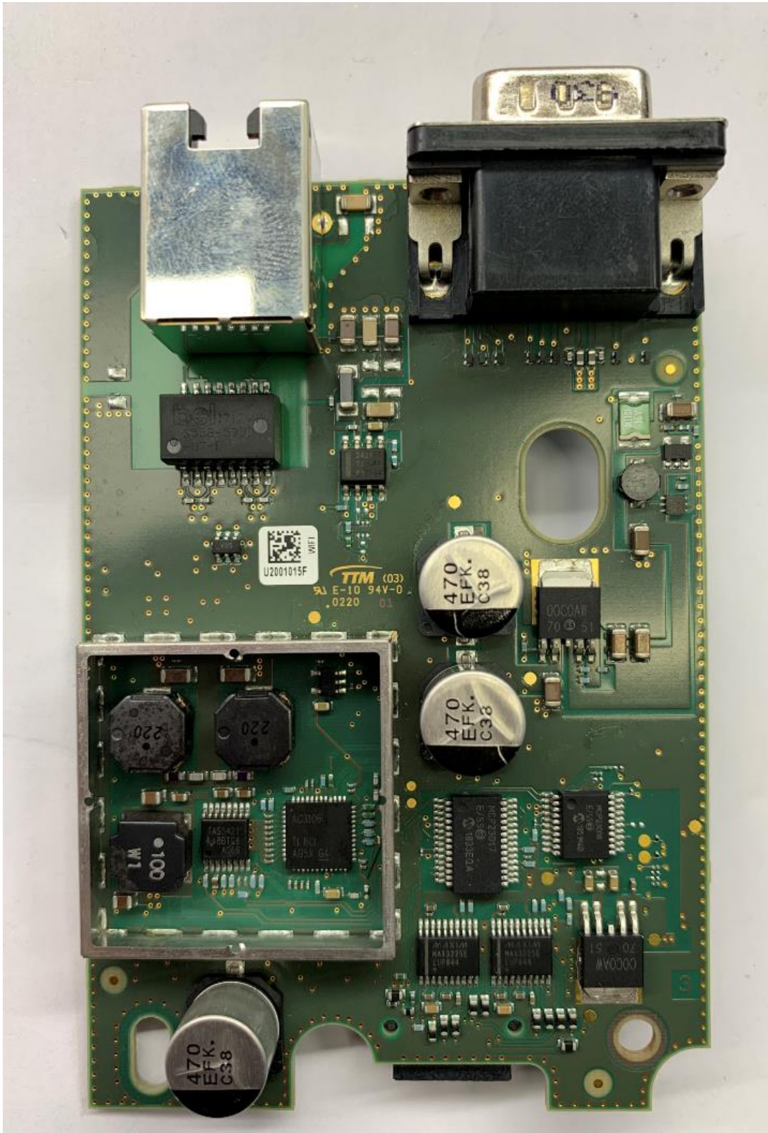
Figure 6. SCG2229 / XX6SCG2229 / 8739A-SCG2229 Expansion Board Top (Can Removed)
