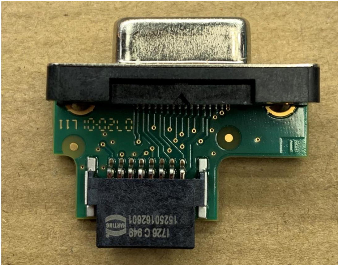
Figure 8. SCG2229 / XX6SCG2229 / 8739A-SCG2229 FC2 RC4 Board Top
