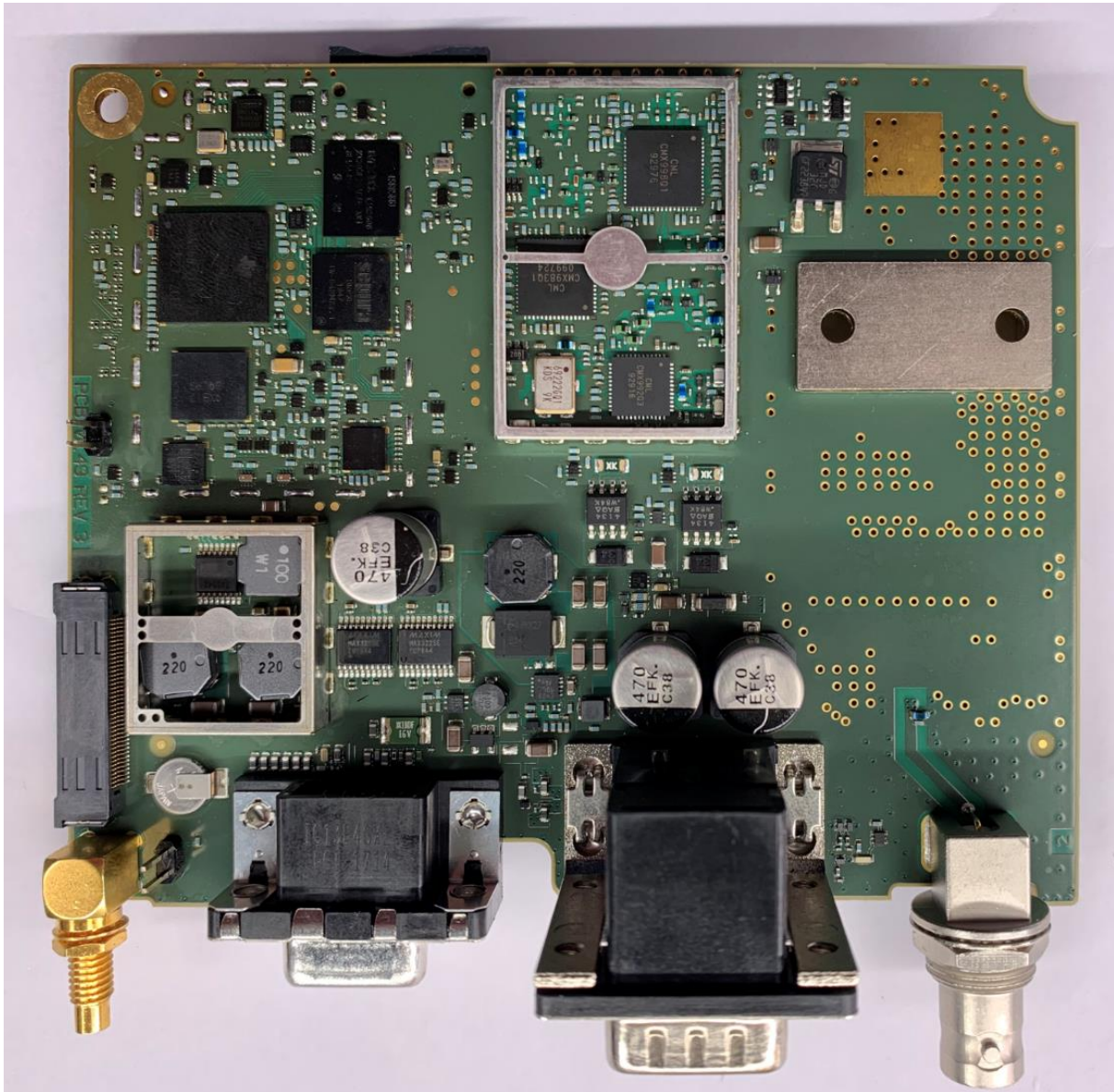
Figure 4. SCG2229 / XX6SCG2229 / 8739A-SCG2229 Main Board Top cans removed
