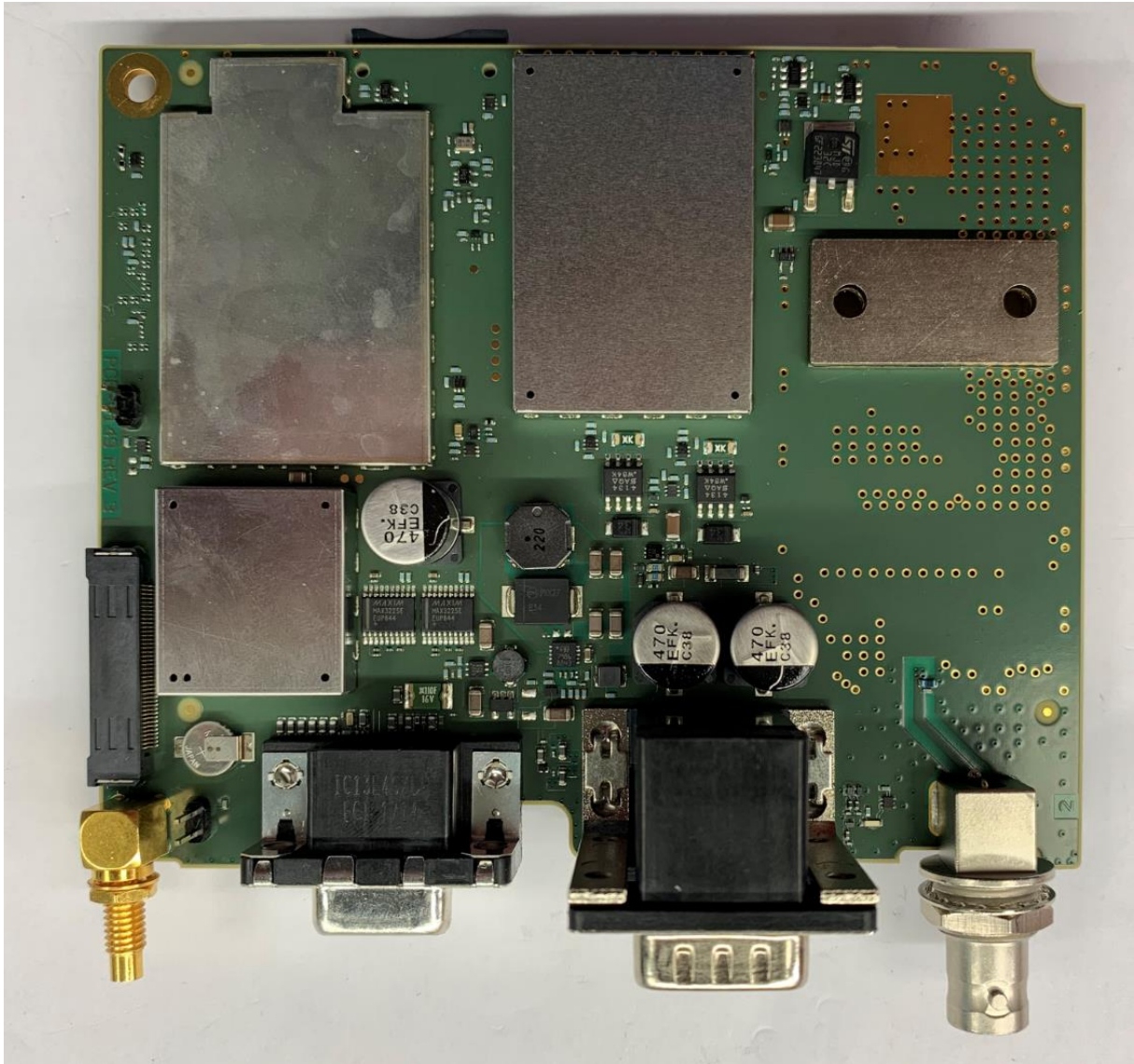
Figure 3. SCG2229 / XX6SCG2229 / 8739A-SCG2229 Main Board Top
