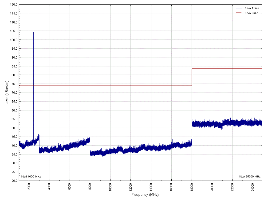
Figure 19 - 2440 MHz - 1 GHz to 25 GHz, Vertical, X Orientation X - Peak
