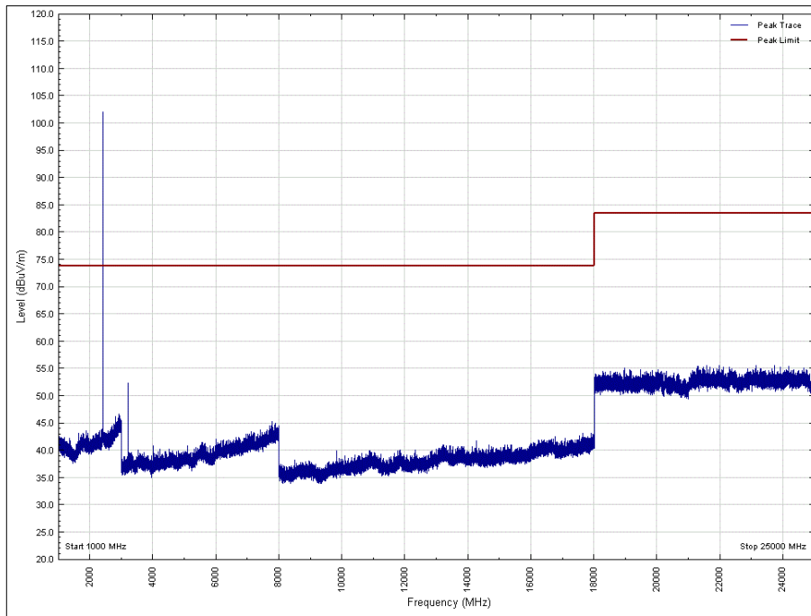
Figure 13 - 2402 MHz, 1 GHz to 25 GHz, Vertical, X Orientation - Peak
