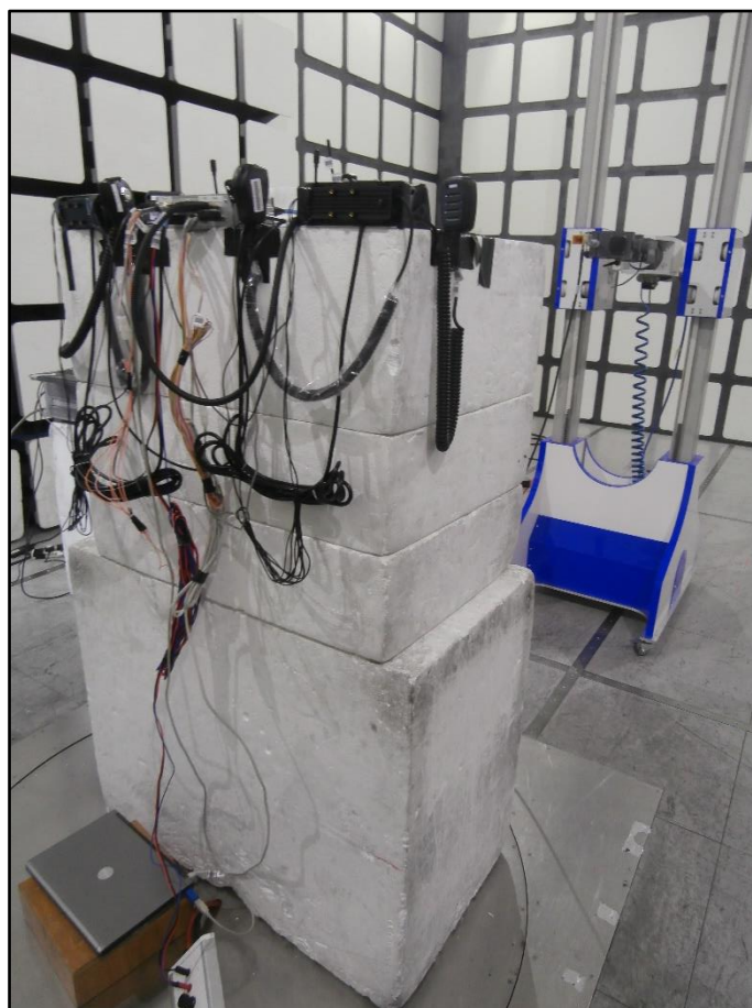
Figure 32 - Test Setup – 18 GHz to 25 GHz (Left View) – X Orientation
