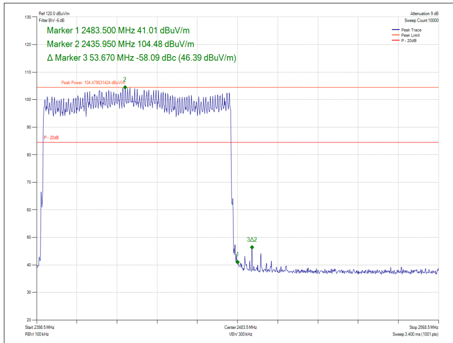
Figure 19 - Hopping - 8-DPSK/3DH5, 2480 MHz - Measured Frequency 2483.5 MHz
