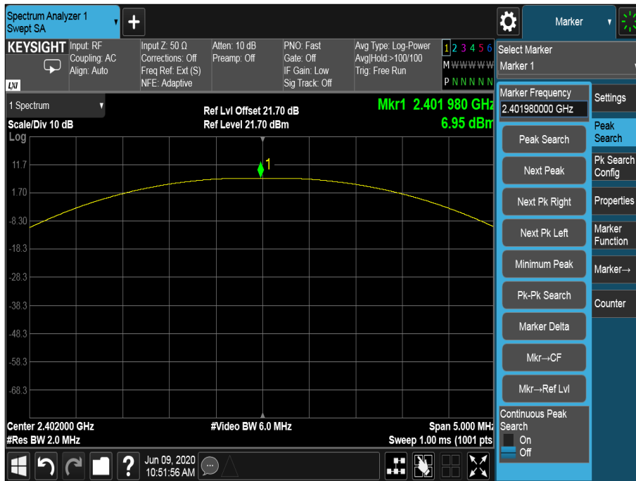
Figure 1 - 2402 MHz, GFSK
