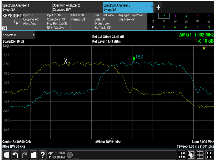
Figure 21 - \pi/4 DQPSK
