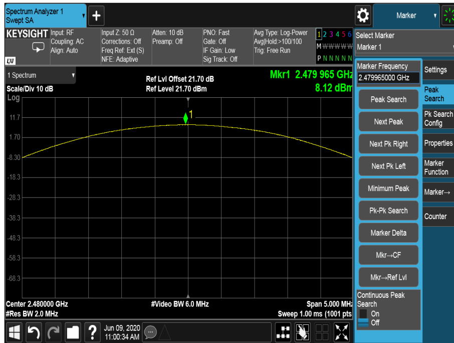
Figure 9 - 2480 MHz, 8-DPSK
