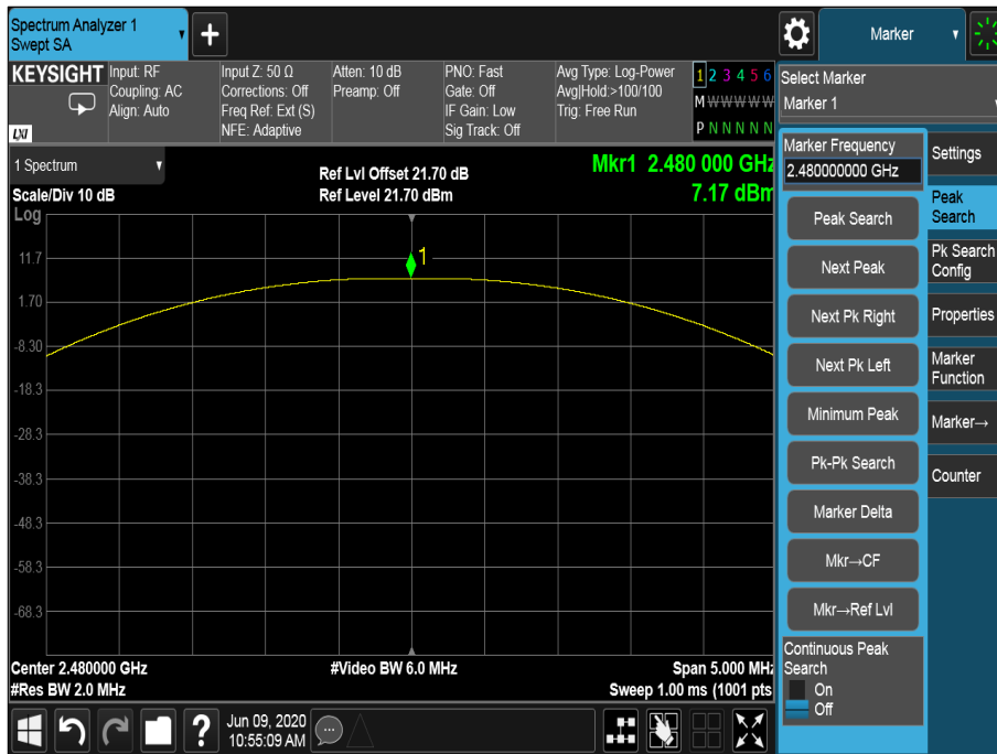
Figure 7 - 2480 MHz, GFSK
