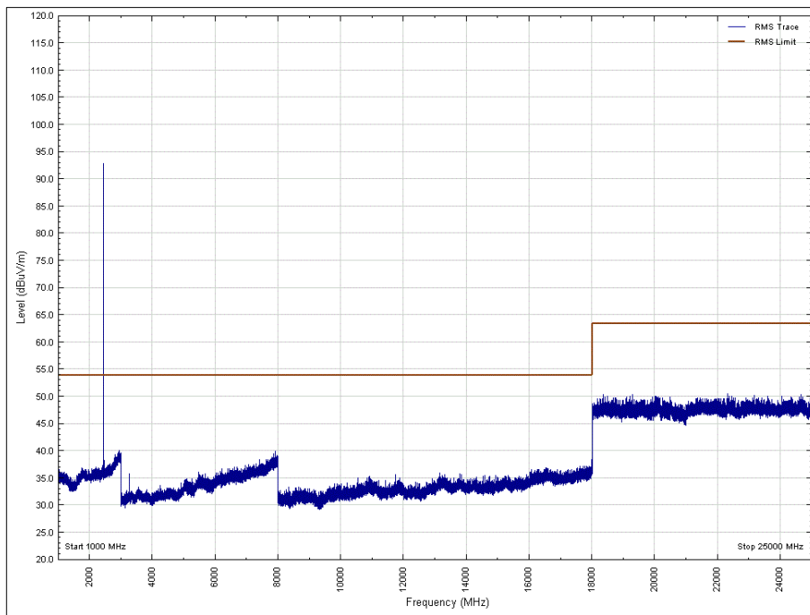
Figure 50 - 2440 MHz - 1 GHz to 25 GHz, Horizontal, X Orientation - Average
