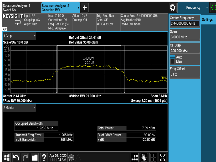
Figure 28 - 2440 MHz - 8-DPSK
