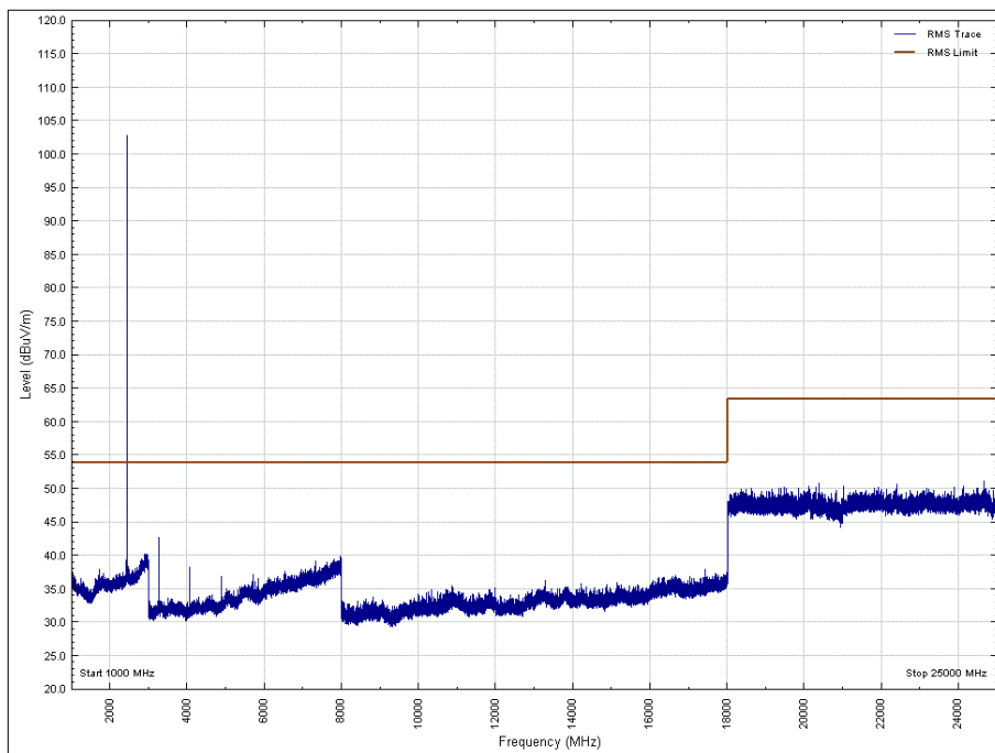
Figure 48 - 2440 MHz - 1 GHz to 25 GHz, Vertical, X Orientation - Average
