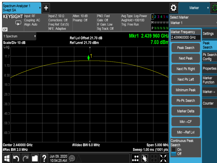
Figure 4 - 2440 MHz, GFSK
