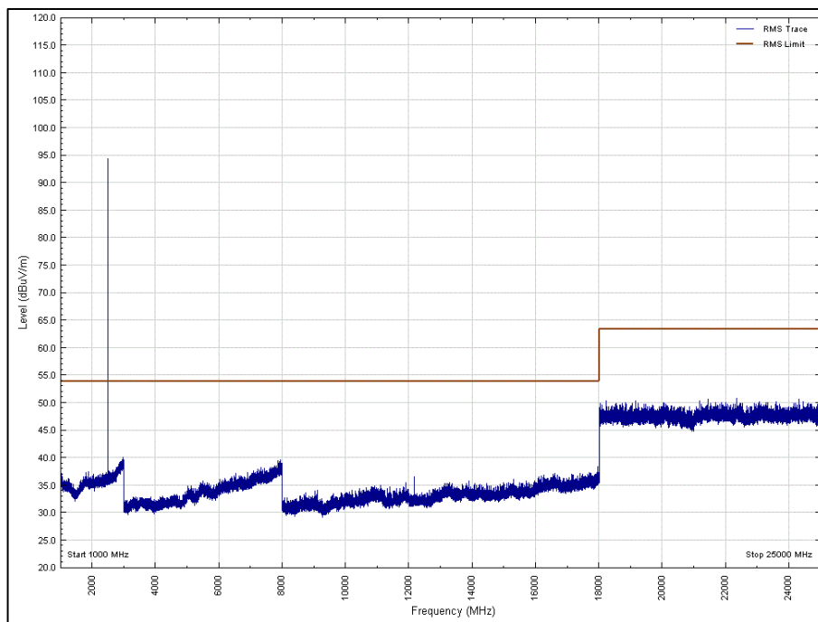
Figure 56 - 2480 MHz – 1 GHz to 25 GHz, Horizontal, X Orientation - Average
