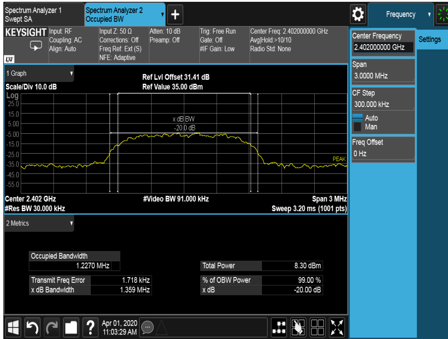
Figure 25 - 2402 MHz - 8-DPSK
