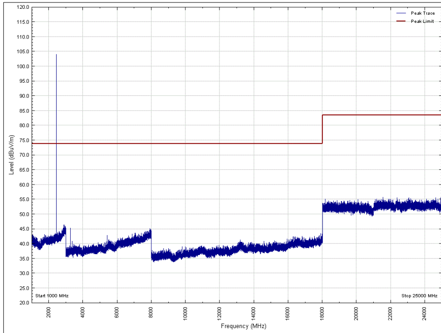
Figure 47 - 2440 MHz - 1 GHz to 25 GHz, Vertical, X Orientation - Peak
