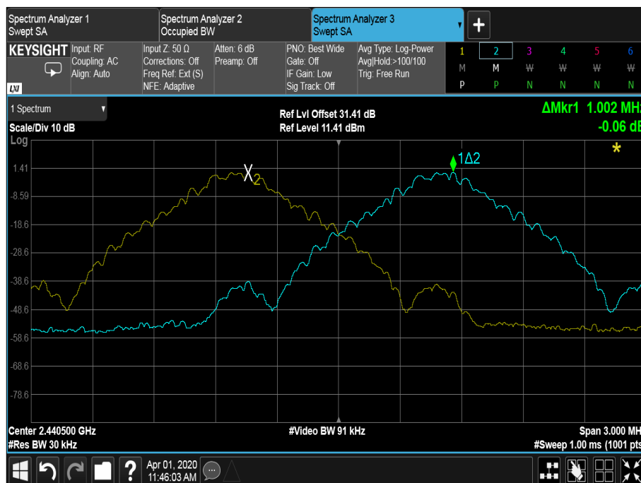
Figure 20 - GFSK
