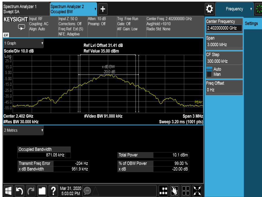
Figure 23 - 2402 MHz - GFSK
