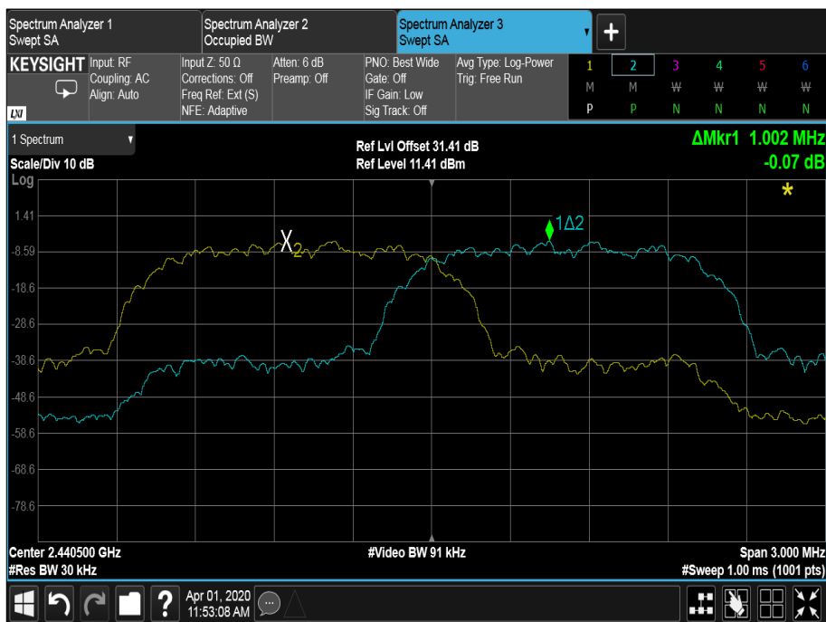
Figure 22 - 8-DPSK
