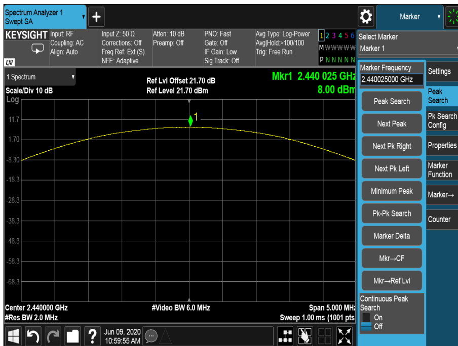
Figure 6 - 2440 MHz, 8-DPSK
