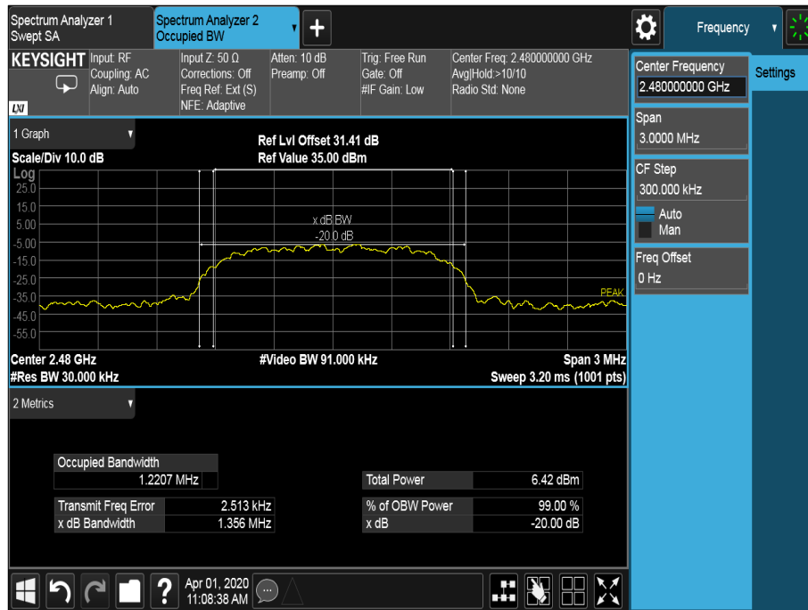
Figure 31 - 2480 MHz - 8-DPSK
