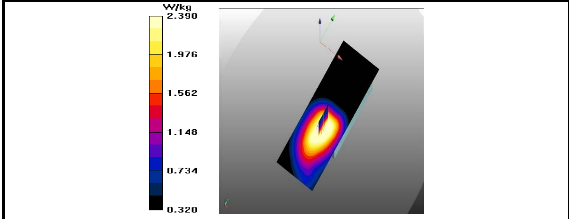
Figure 31: SAR Body Testing Results for the SC2128 TETRA Radio at 815 MHz
