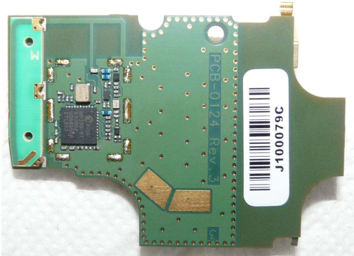
Figure 10. SC2128 GPS Module Front View With Can Removed
