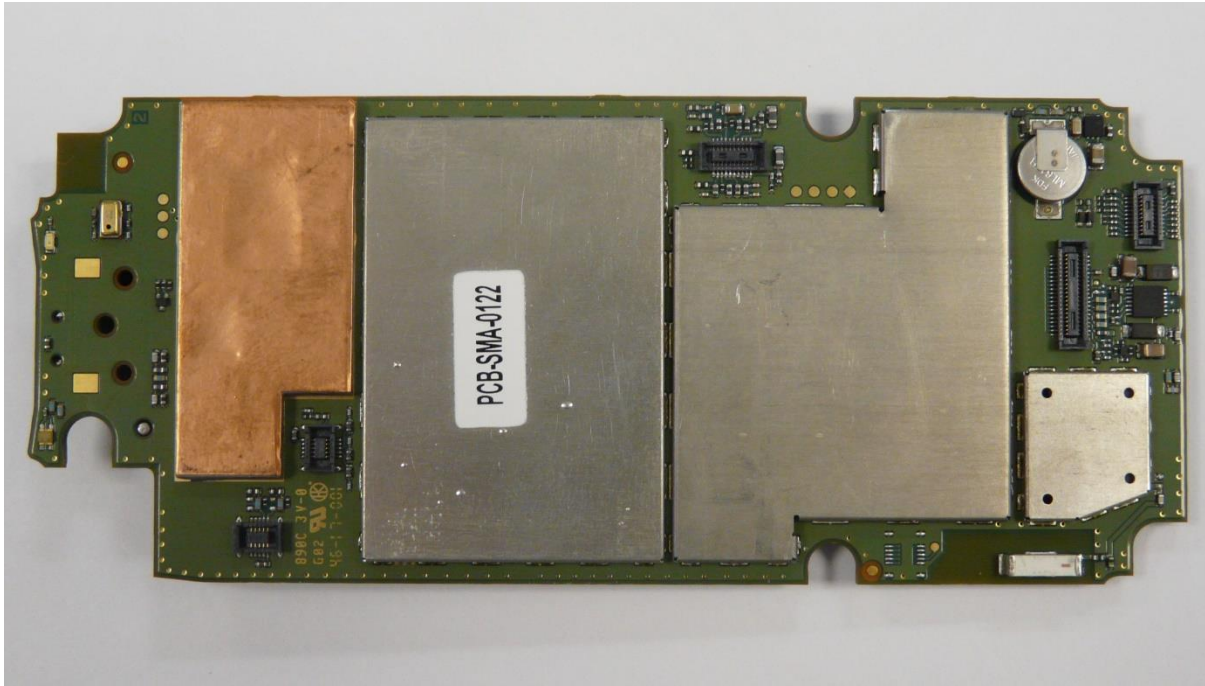
Figure 3. SC2128 Main PCB Rear View
