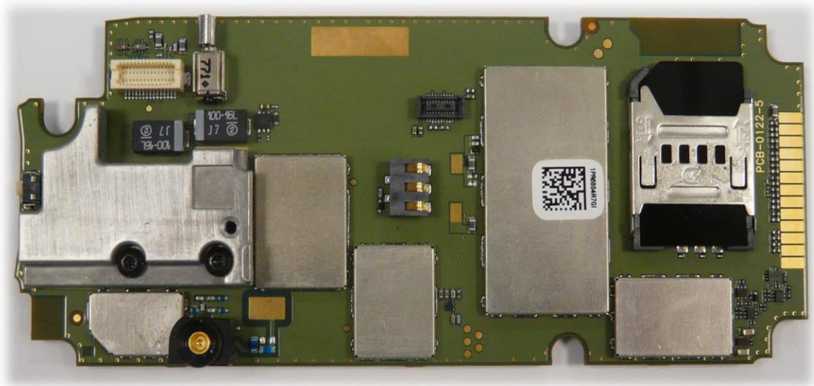
Figure 4. SC2128 Main PCB Rear View With GPS Module Removed
