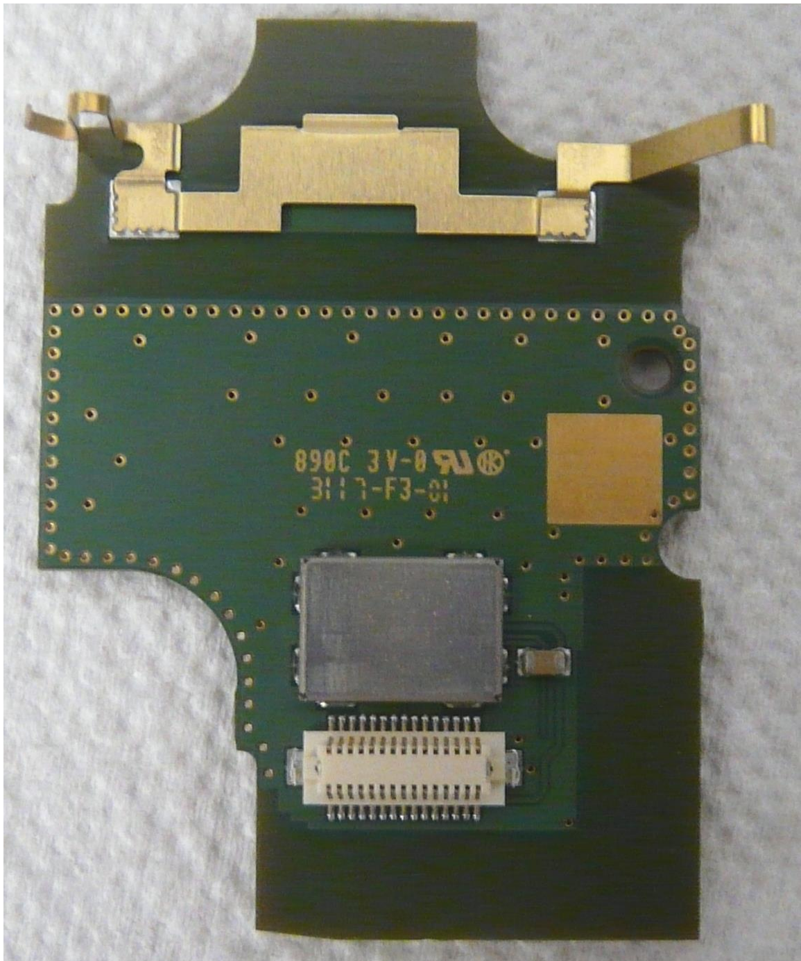
Figure 5. SC2128 GPS Module Rear View
