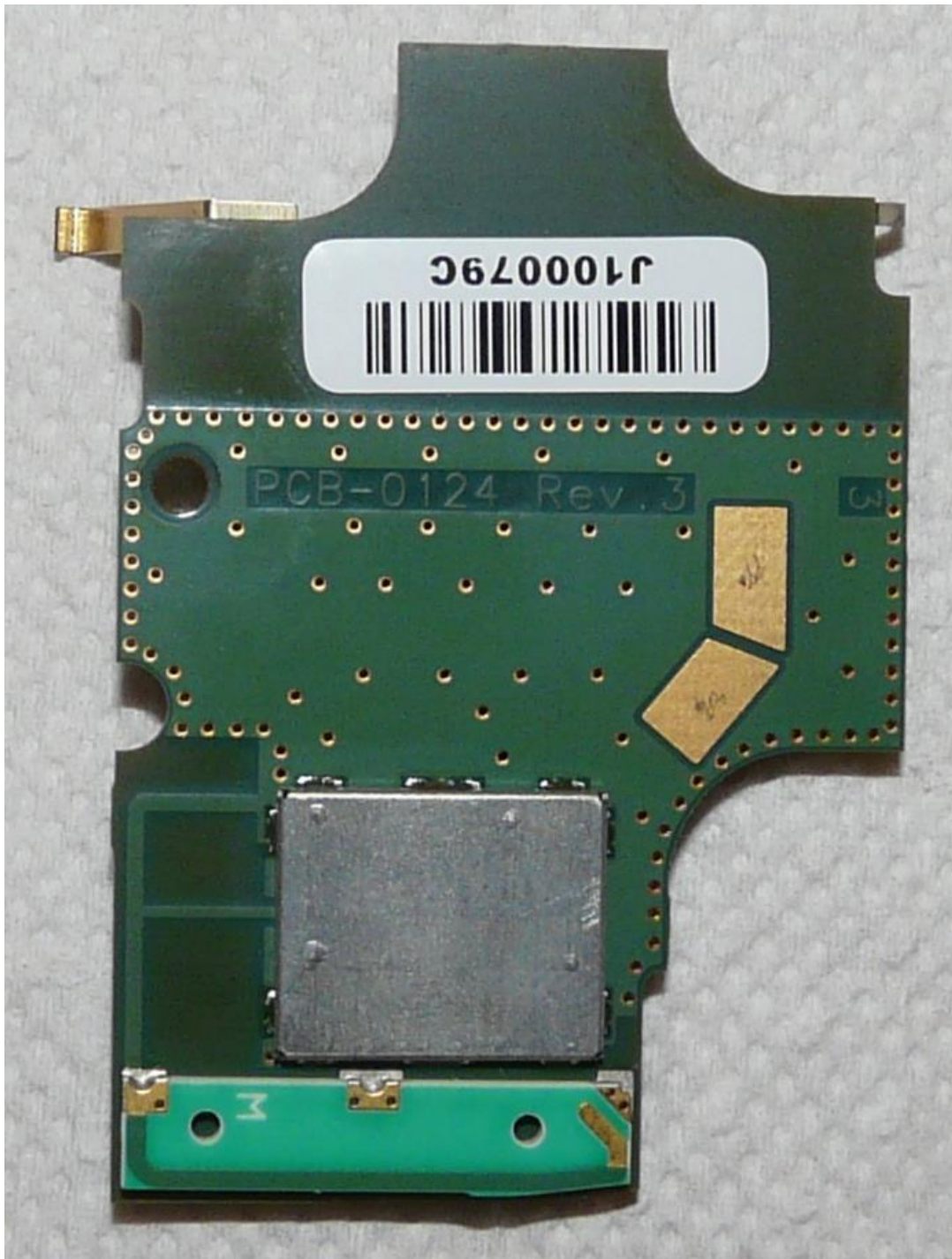
Figure 6. SC2128 GPS Module Front View
