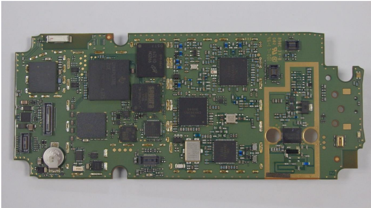
Figure 8. SC2128 Main PCB Rear View With Cans Removed
