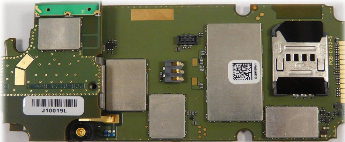
Figure 3. SC2128 Main PCB Rear View
