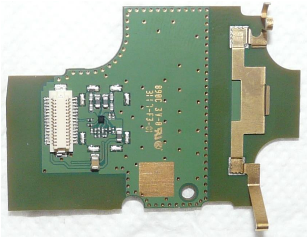
Figure 9. SC2128 GPS Module Rear View With Can Removed
