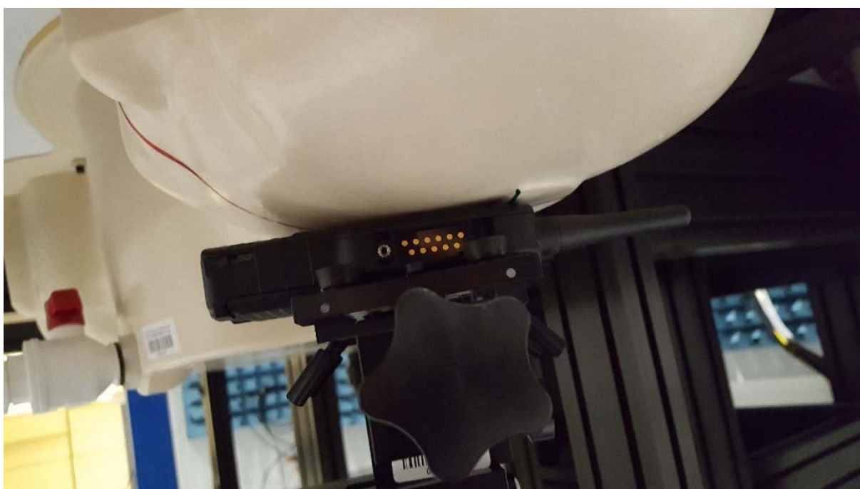
SAR - Head - Left Cheek - 1160 mAh Battery
