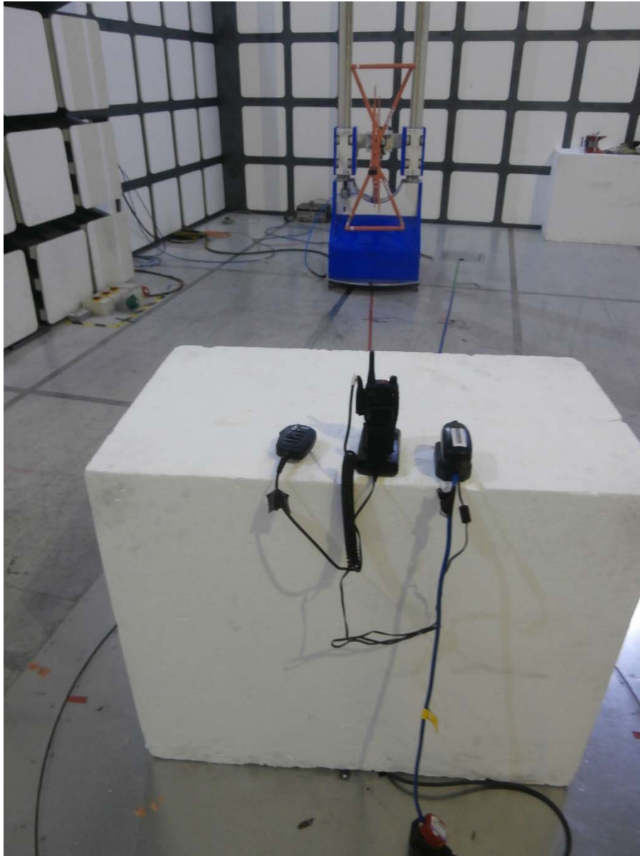
FCC Part 15.247 Radiated Emissions 30 MHz to 1 GHz
