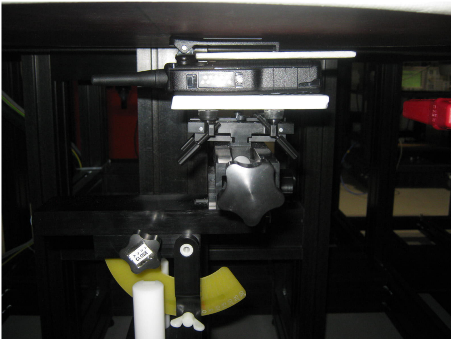
Figure 59 Rear Face - 1160 mAh Battery (Part no: 300-01852) Extended Helical Antenna (Part no: 300-01960) 0 mm Separation distance
