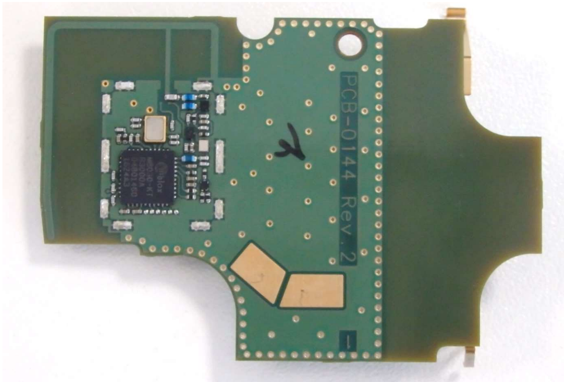
Figure 10. XX6SC2124 GPS Module Front View with Can Removed
