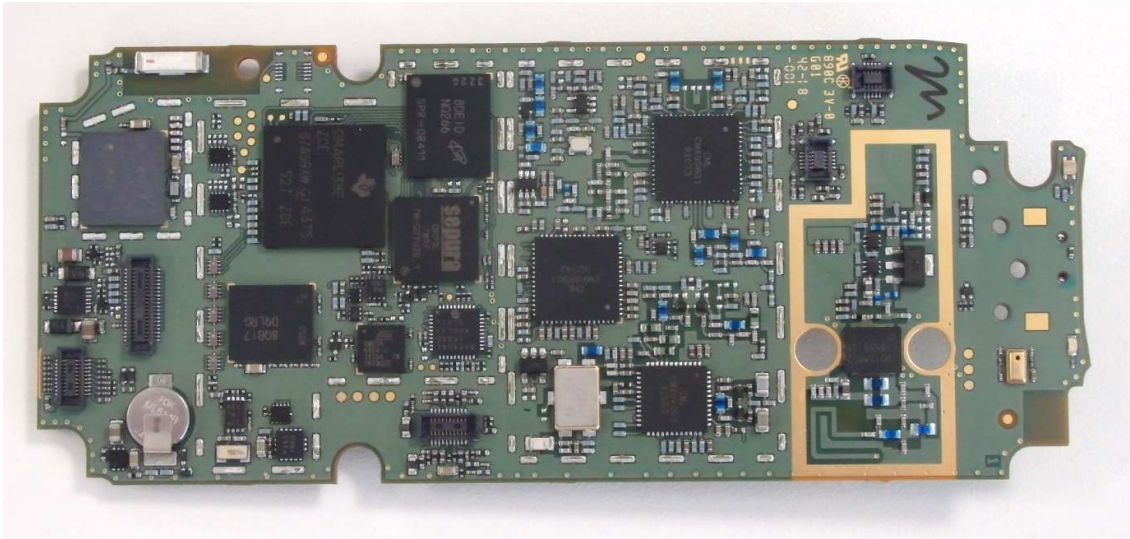
Figure 7. XX6SC2124 Main Board Front View with Cans Removed
