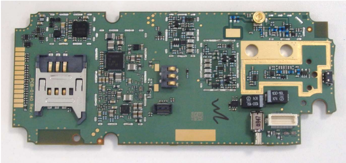
Figure 8. XX6SC2124 Main Board Rear View with Cans Removed
