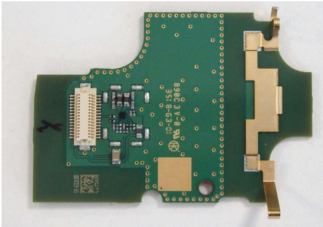
Figure 9. XX6SC2124 GPS Module Rear View with Can Removed
