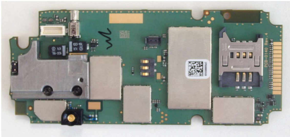
Figure 4. XX6SC2124 Main PCB Rear View with GPS Removed
