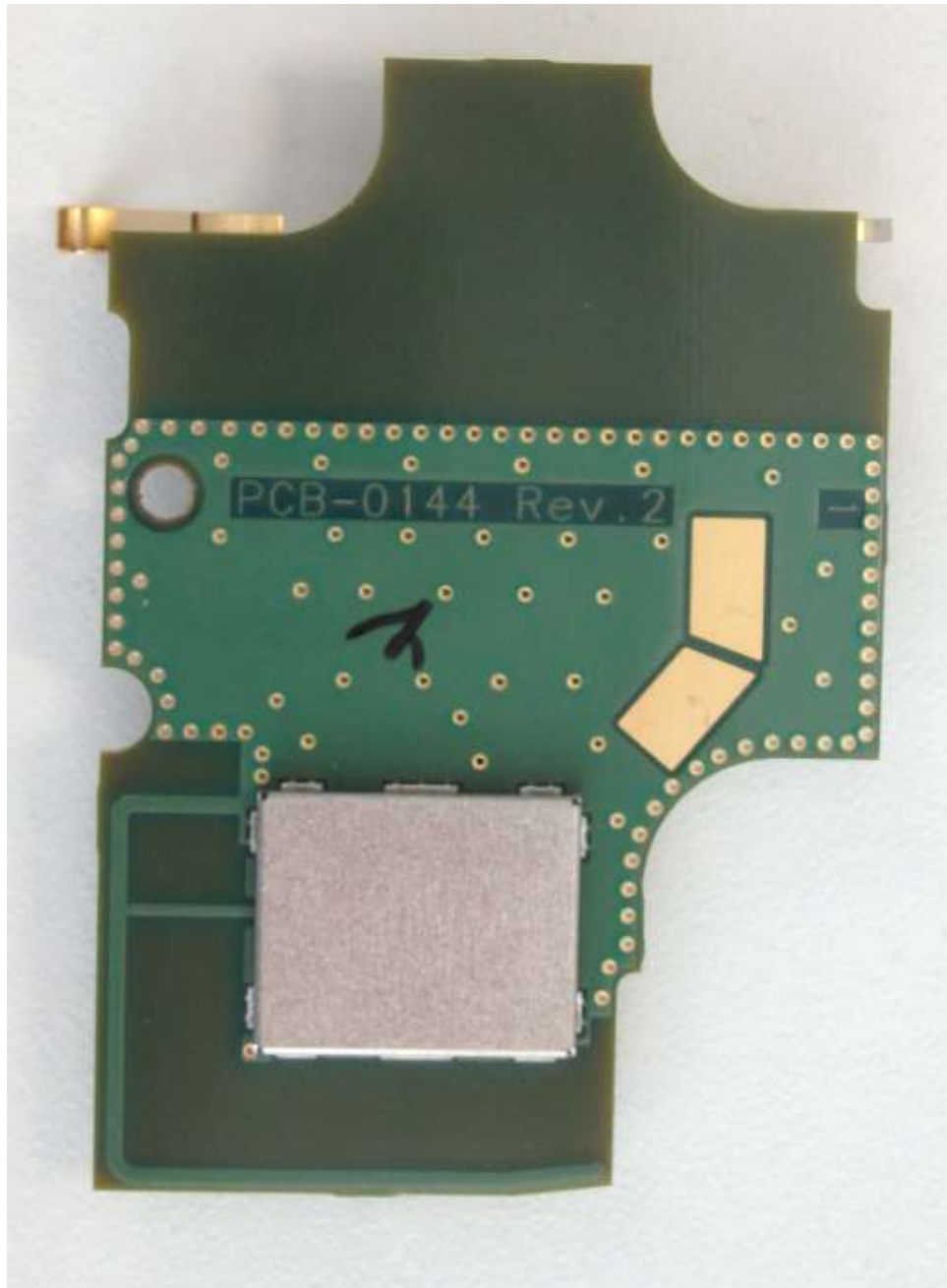
Figure 6. XX6SC2124 GPS Module Front View
