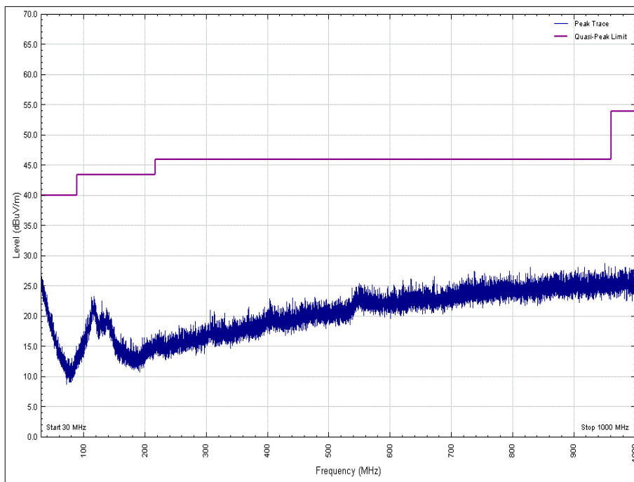
Figure 17 - 2402 MHz - 30 MHz to 1 GHz, Polarity: Horizontal, EUT Orientation: X
