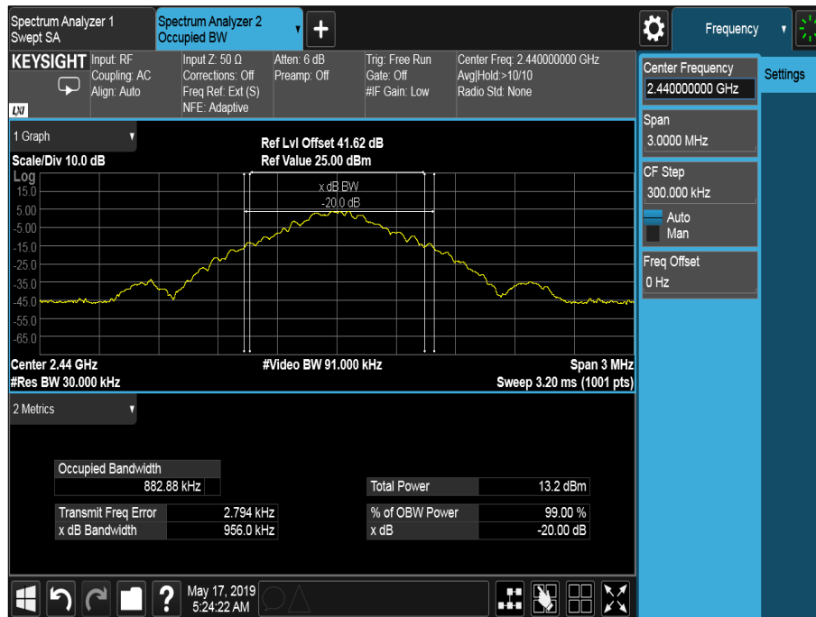
Figure 20 - 2440 MHz - GFSK
