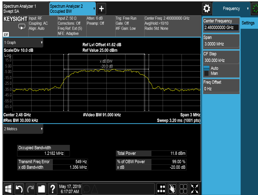
Figure 25 - 2480 MHz - 8-DPSK
