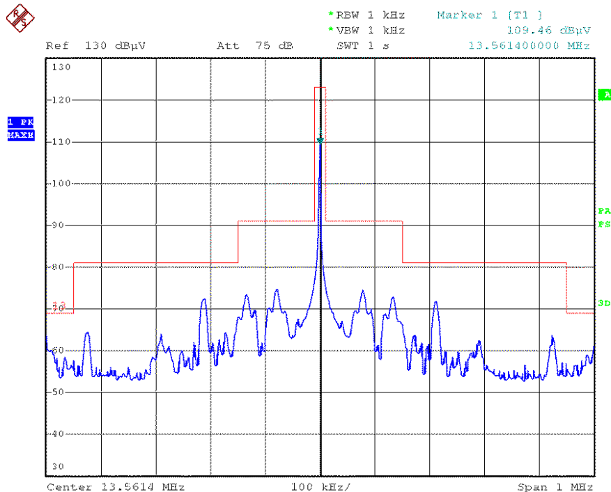
Figure 5: Spectrum Mask
