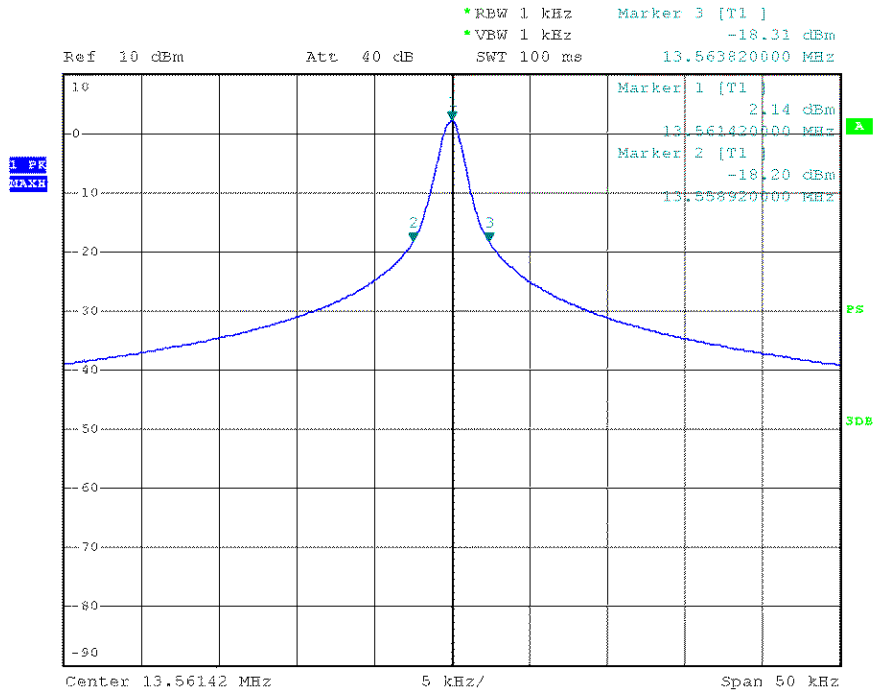
Figure 6: Occupied bandwidth
