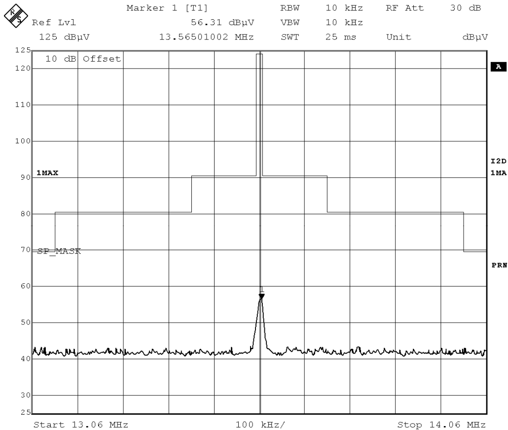
Figure 6: Spectrum Mask
