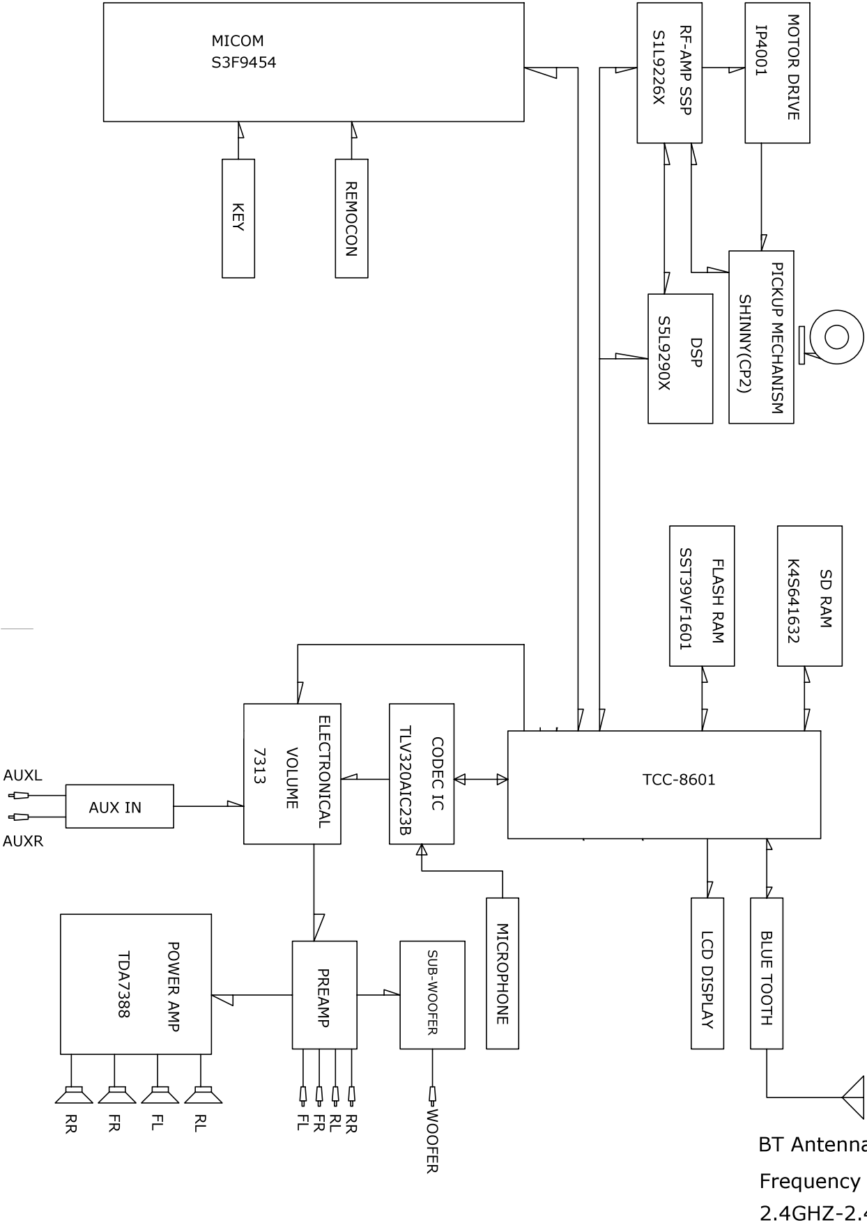
BLOCK DIAGRAM
