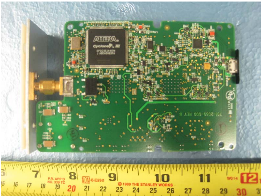
EUT Cover off Component view
