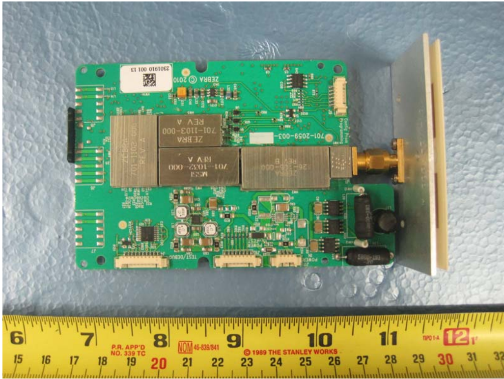
EUT Cover off Solder view
