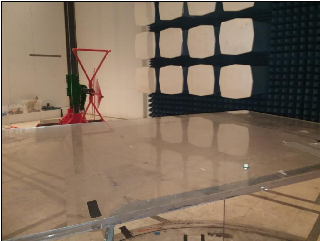
Photograph 2. Radiated Emissions, Below 1 GHz, Test Setup
