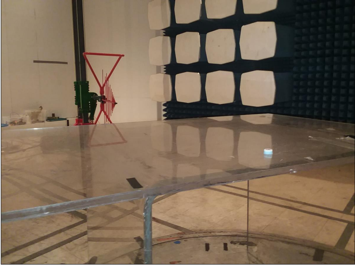
Photograph 2. Radiated Emissions below 1GHz, Test Setup
