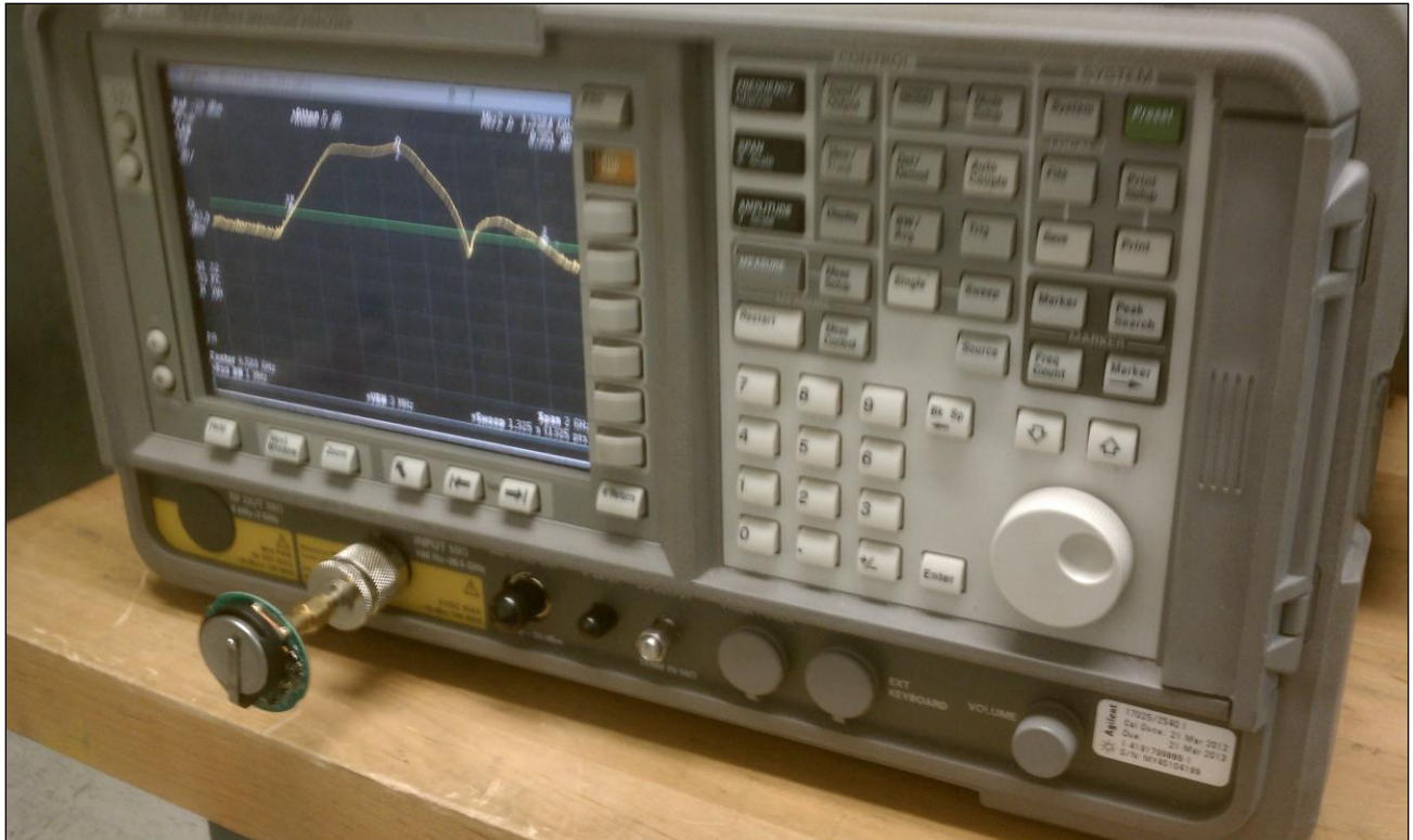
Photograph 4. GPS Bands, Test Setup
