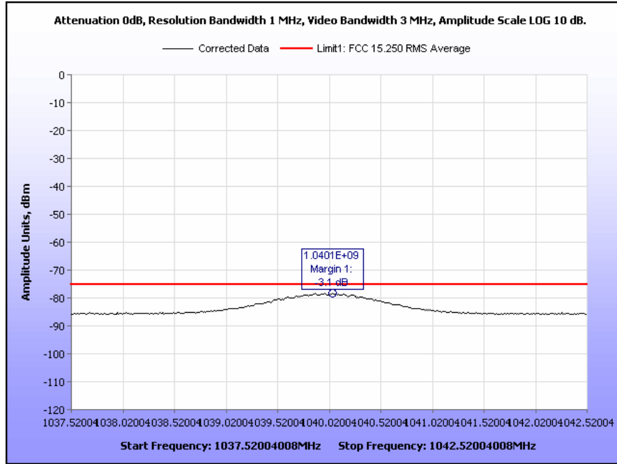
Plot 7. Radiated Emissions Above 960 MHz, 1.040 GHz Emission, Average
