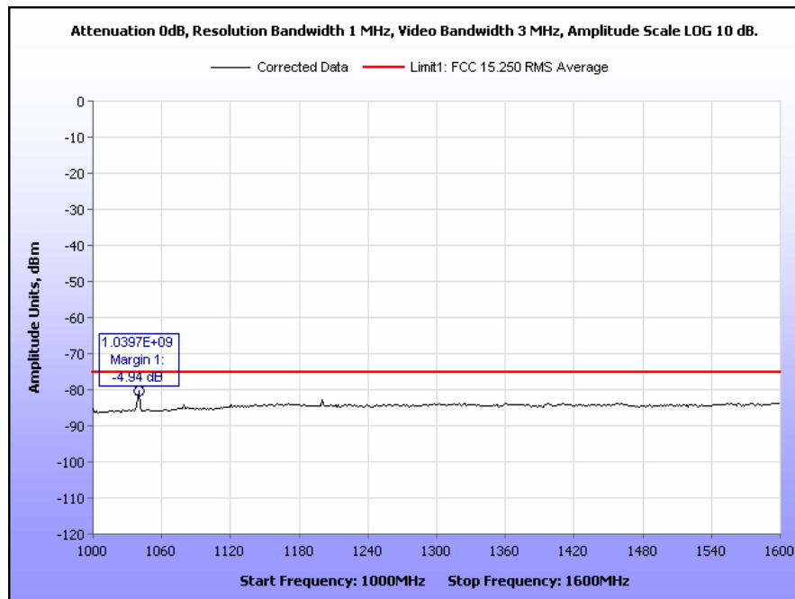
Plot 6. Radiated Emissions Above 960 MHz, 1 GHz – 1.6 GHz, Average
