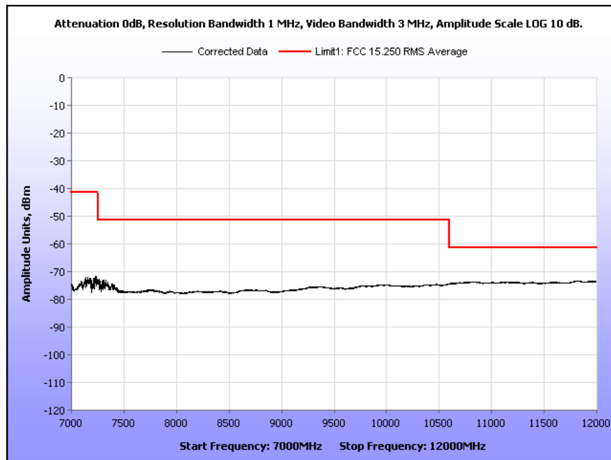
Plot 10. Radiated Emissions Above 960 MHz, 7 GHz – 12 GHz
