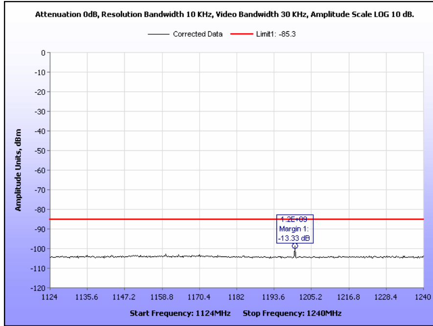
Plot 12. GPS Bands, 1.124 GHz – 1.240 GHz, Average
