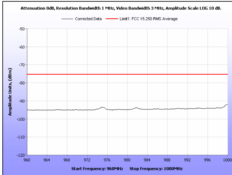
Plot 5. Radiated Emissions Above 960 MHz, 960 MHz – 1 GHz
