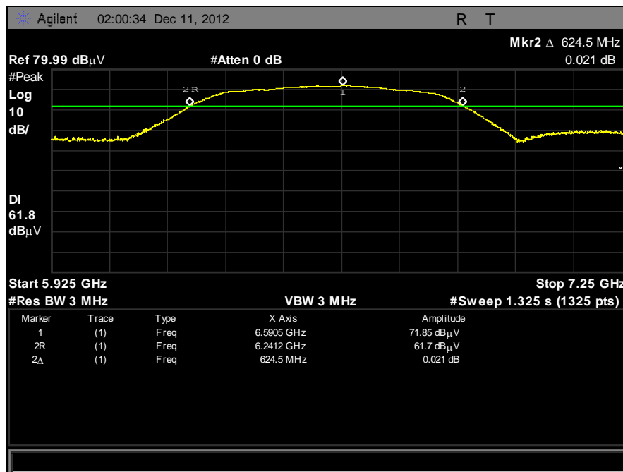
Plot 3. -10 dB Bandwidth
