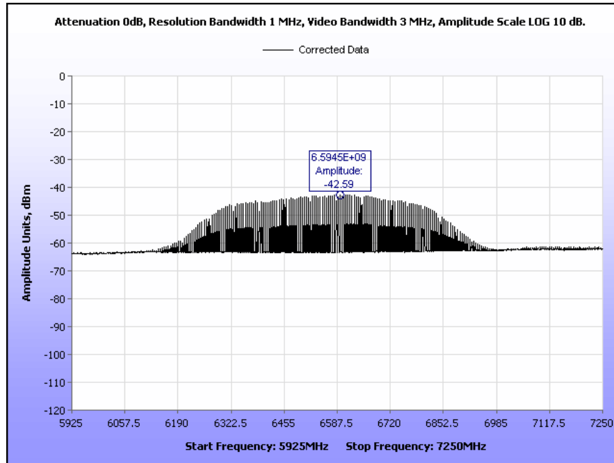
Plot 9. Radiated Emissions Above 960 MHz, 5.925 GHz – 7.250 GHz, Average
