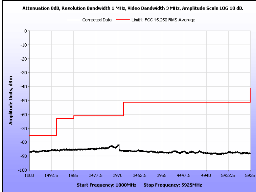
Plot 8. Radiated Emissions Above 960 MHz, 1 GHz – 5.925 GHz
