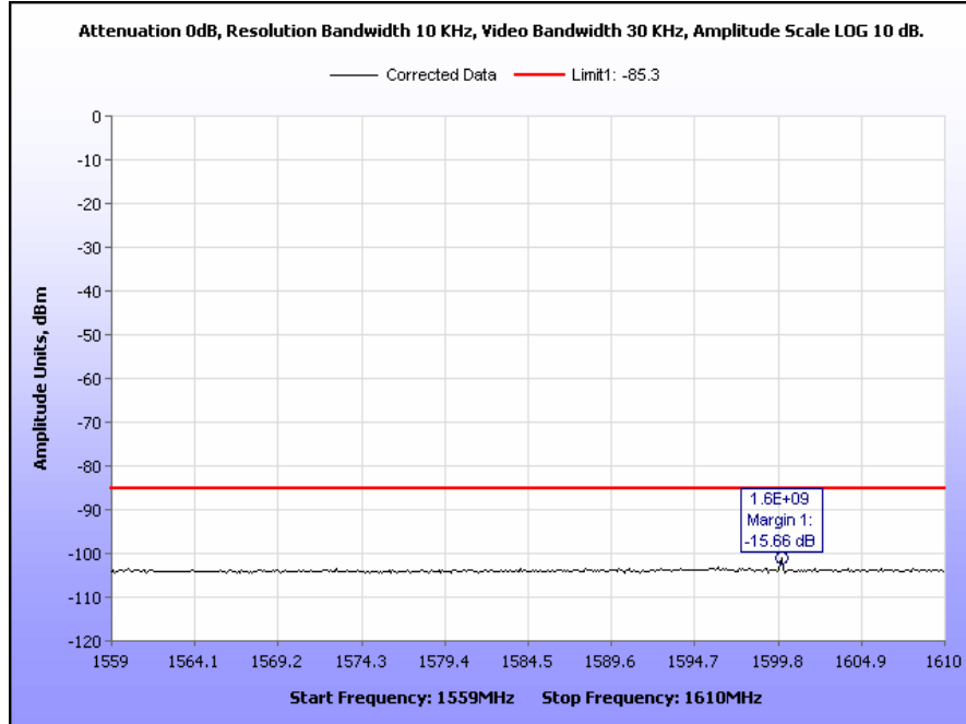
Plot 13. GPS Bands, 1.559 GHz – 1.610 GHz, Average
