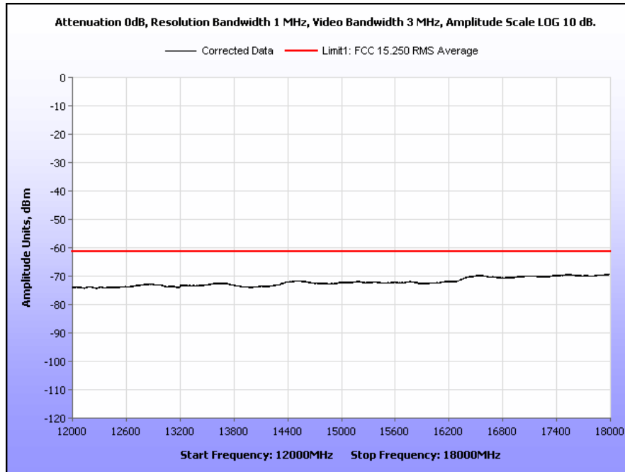
Plot 11. Radiated Emissions Above 960 MHz, 12 GHz – 18 GHz
