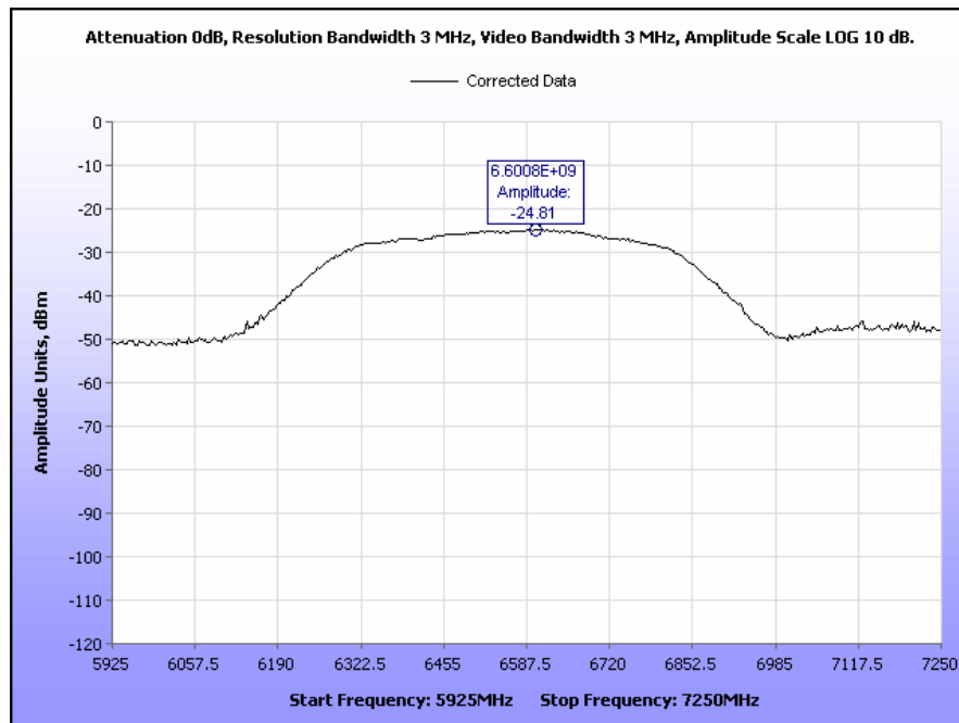
Plot 14. Peak Emissions, 5.925 GHz – 7.250 GHz
