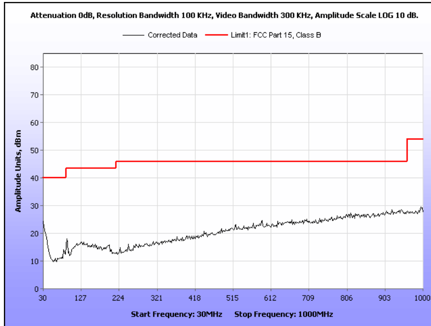
Plot 15. Radiated Emissions Below 960 MHz, 30 MHz – 1 GHz
