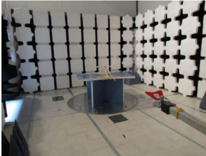
Antenna AK110
