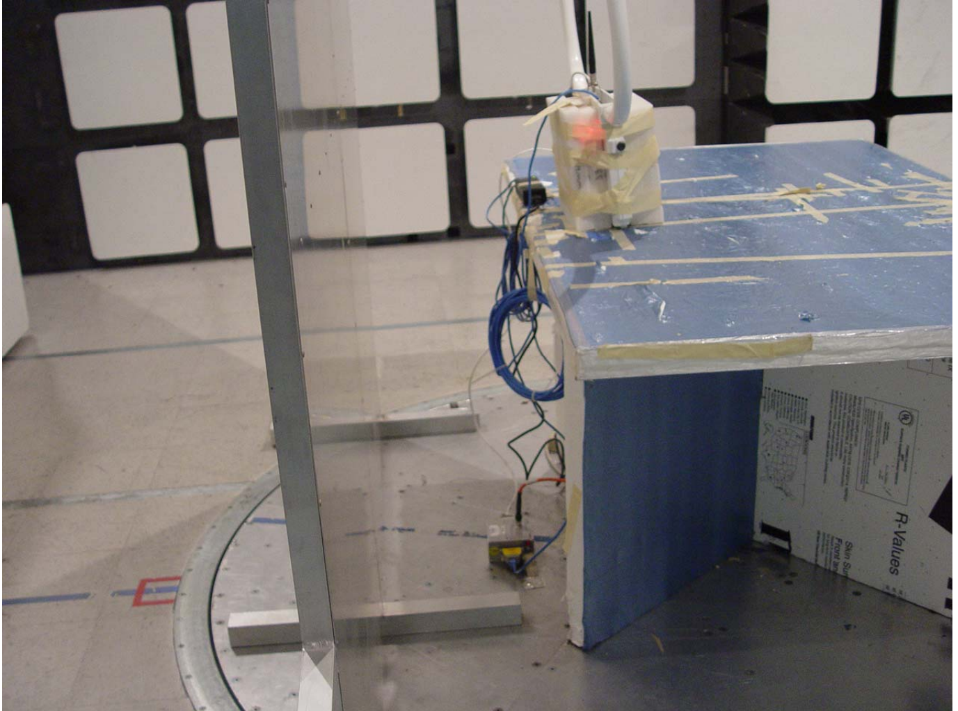
WhereLAN III Location Sensor, model# LOS-5000, conducted measurements , <30MHz
