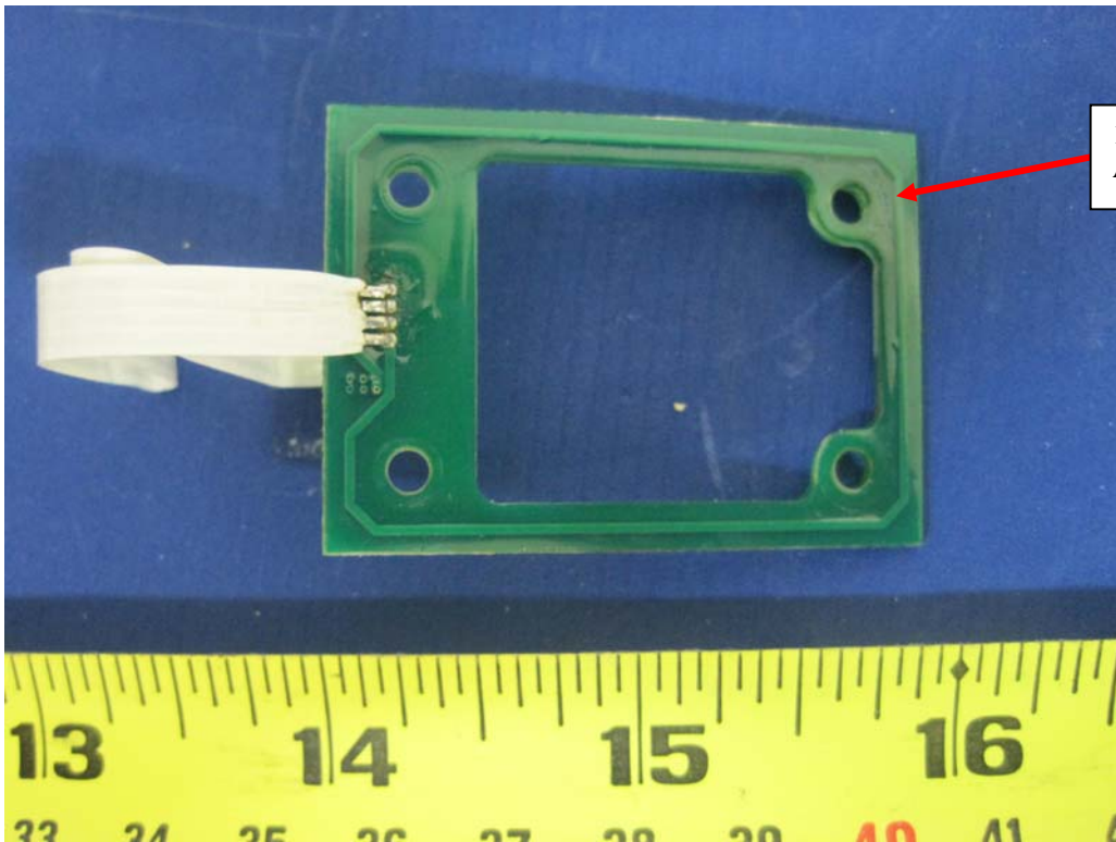
13.56MHz RFID Antenna Solder View
