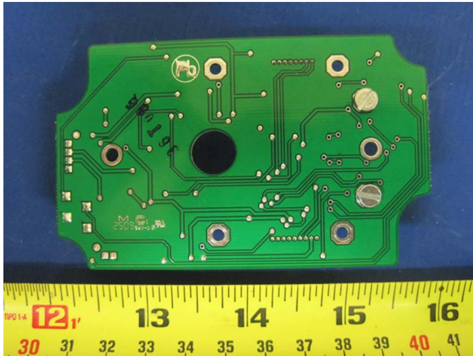
PCBA2 Bottom View
