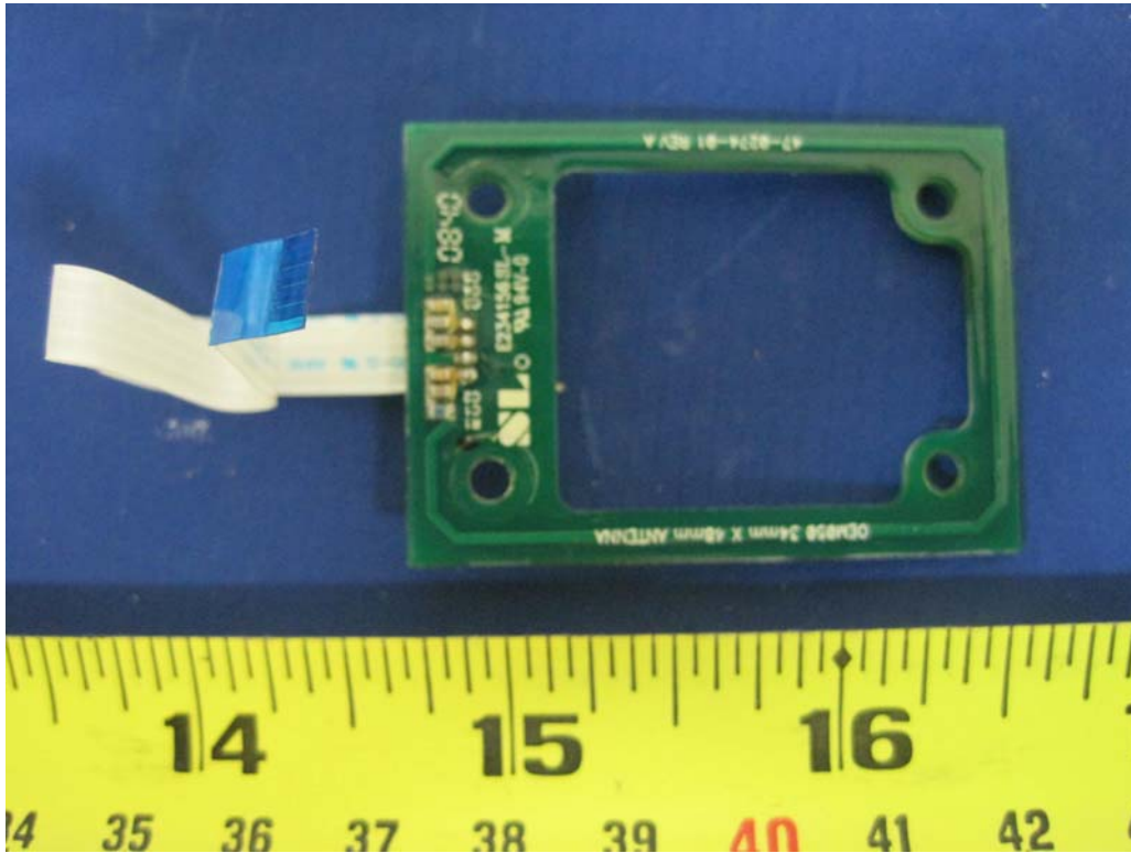
13.56MHz RFID Antenna Component View
