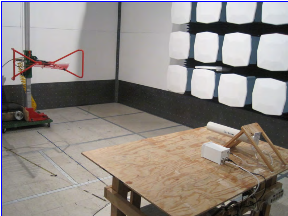
Radiated Emission, AIR-ANT1949 (30 MHz-1 GHz) – Rear View
