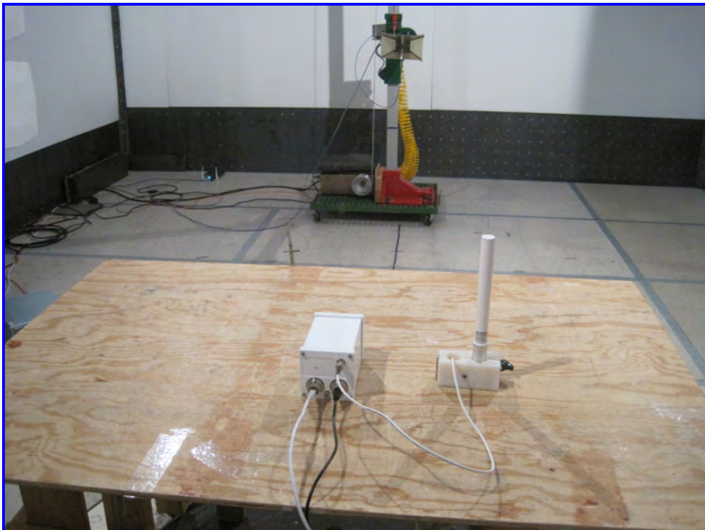
Radiated Emission, AIR-ANT2506 (Above 1 GHz) – Rear View
