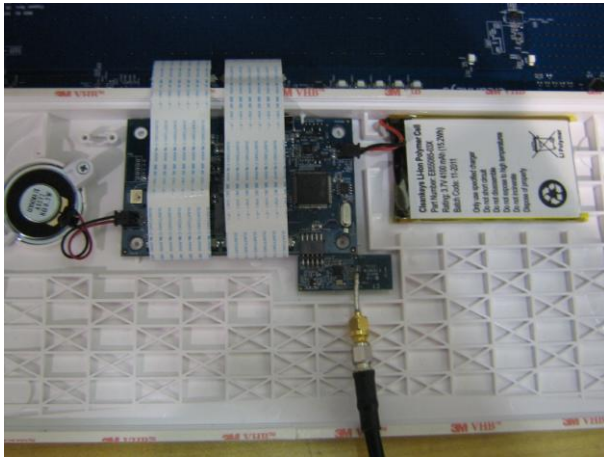
Figure 6 - Test setup for conducted emissions of CKW module with PPxMnnWx30 host.
