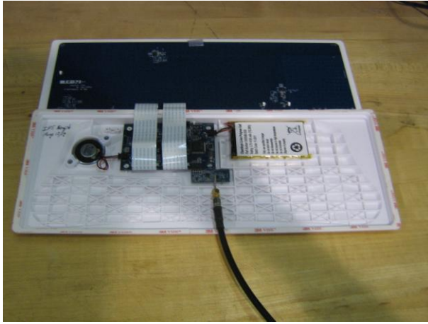
Figures 5 - Test setup for conducted emissions of CKW module with PPxMnnWx30 host.
