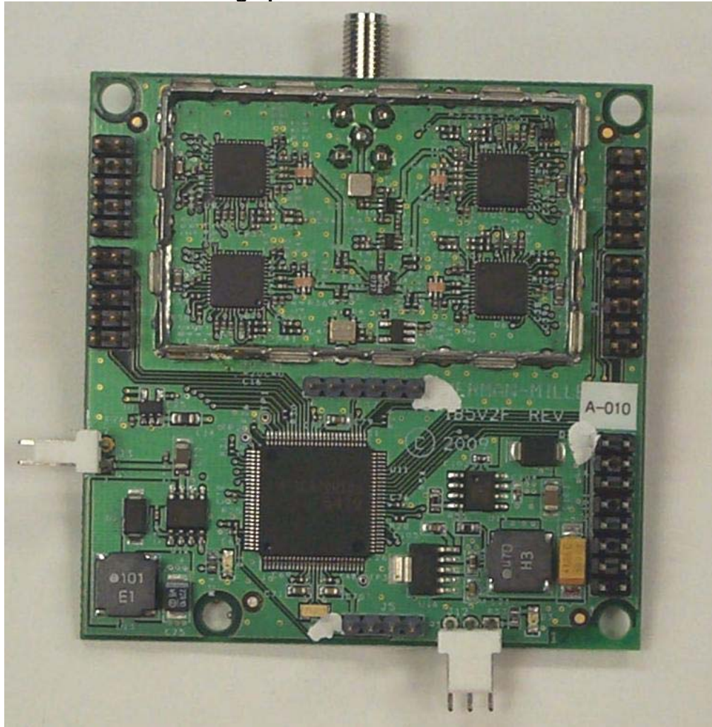
Photograph of EUT Covered removed
