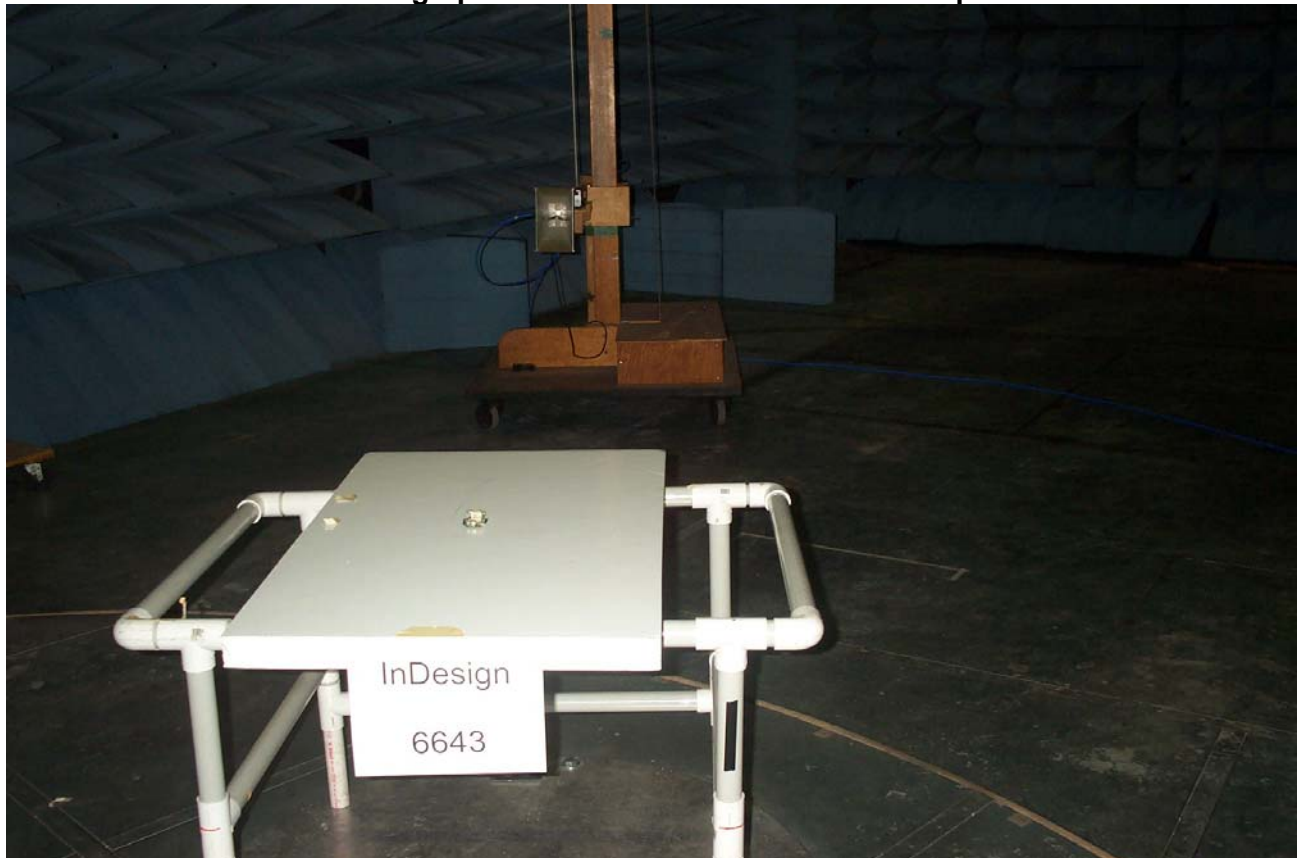
Photograph of Radiated Emissions Test Setup
