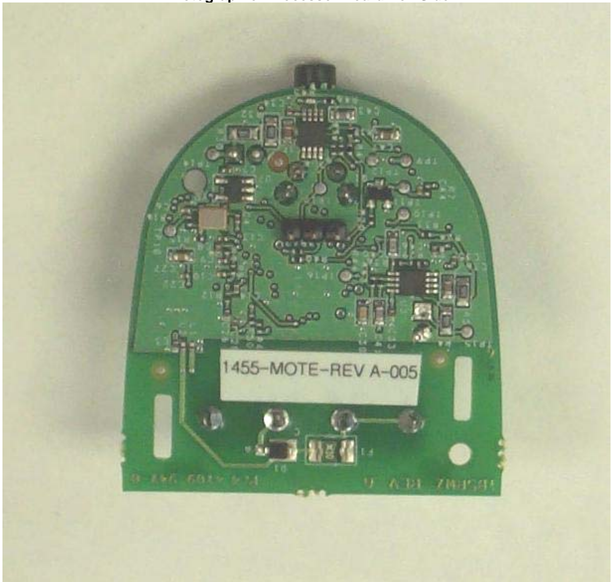
Photograph of Processor Board-Foil Side
