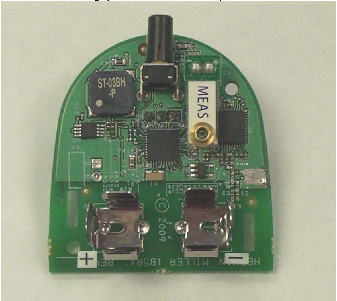
Photograph of Processor Board-Component Side
