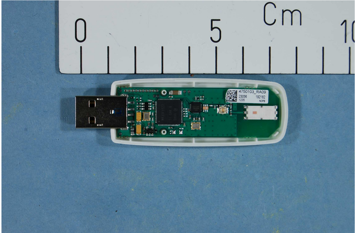
Dosimetry USB Radio (with 50 ohms connector for conducted measurements)
