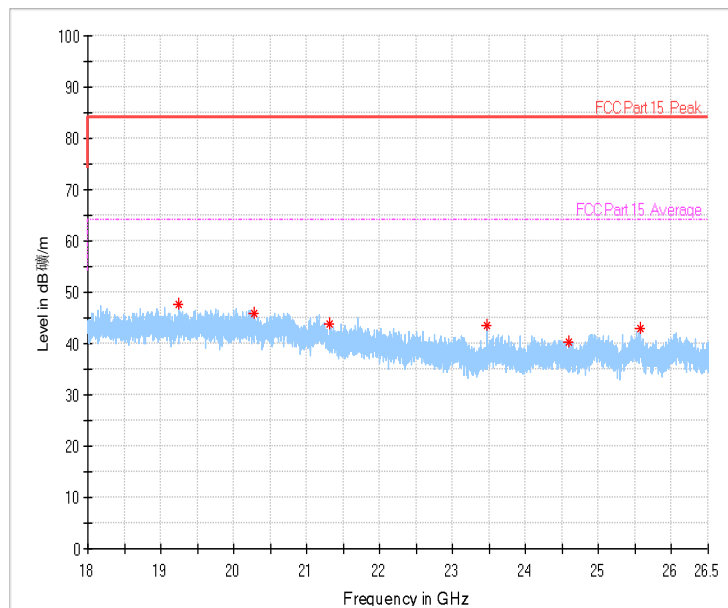
Fig.57 Radiated emission: 8DPSK, 18 GHz - 26 GHz
