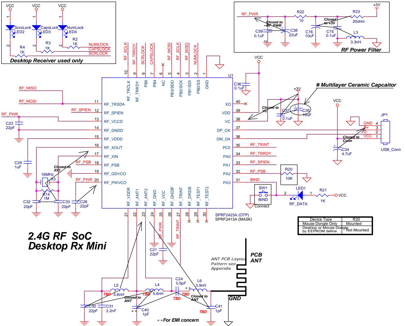
2.4GHz RF SoC Mini Receiver application circuitry
