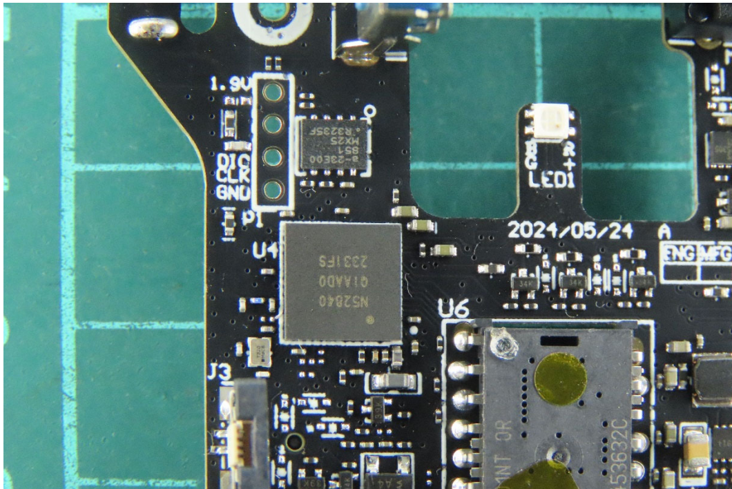
(5) EUT Photo - Brand Name: ASUS, Model No.: P718
