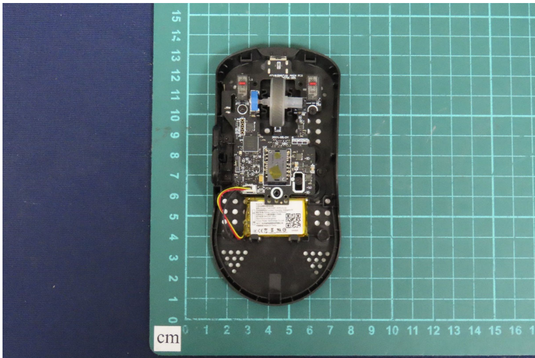
(2) EUT Photo - Brand Name: ASUS, Model No.: P718
