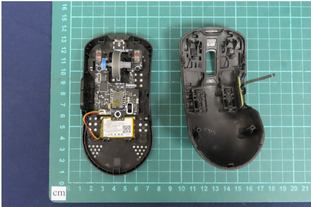
(1) EUT Photo - Brand Name: ASUS, Model No.: P718
