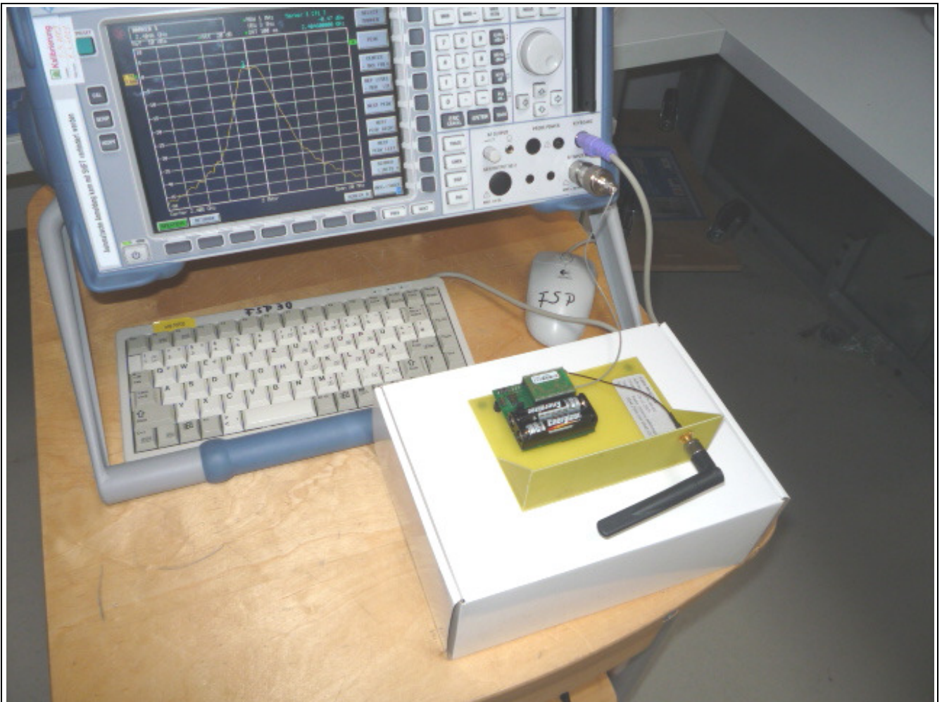
Figure 1: Measurement set-up for conducted measurement acc. following sections of the report 1234-09-EE-10-PB005: 4.1.1; 4.1.2; 4.2; 4.3 and 4.4.3
