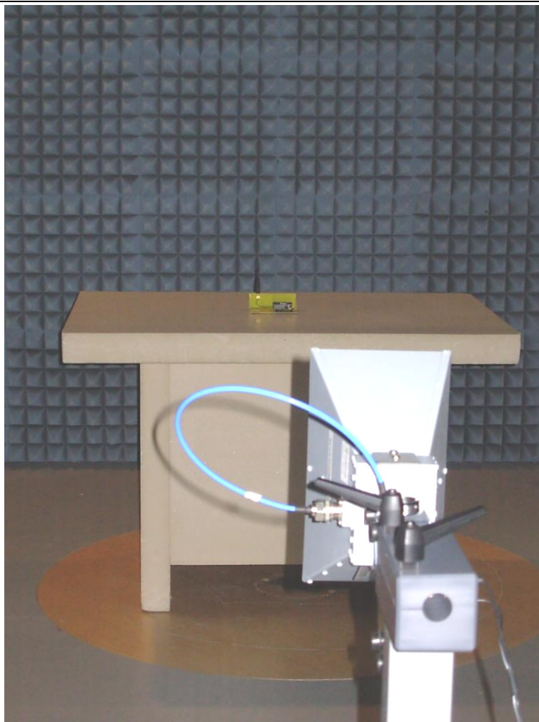
Figure 3: Measurement set-up for radiated measurement > 1 GHz acc. following sections of the report 1234-09-EE-10-PB005: 4.4.2 and 4.5.2
