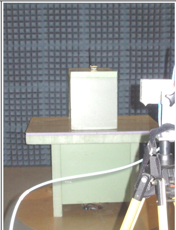
Figure 10: Measurement set-up for radiated measurement > 1 GHz acc. following sections of the report 1113-11-EE-11-PB001: 4.5.3; 4.5.4 and 4.6.2
