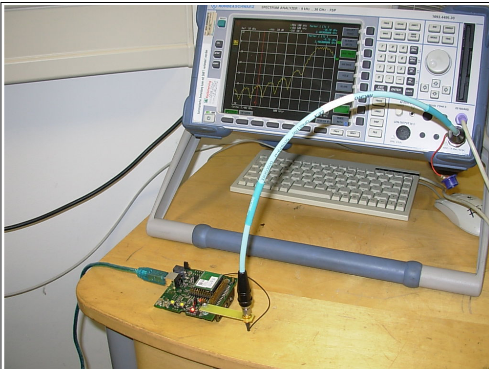
Figure 7: Measurement set-up for conducted measurement acc. to following sections of the report 1113-11-EE-11-PB001: 4.1.1; 4.1.2; 4.2; 4.3; 4.4 and 4.5.5
