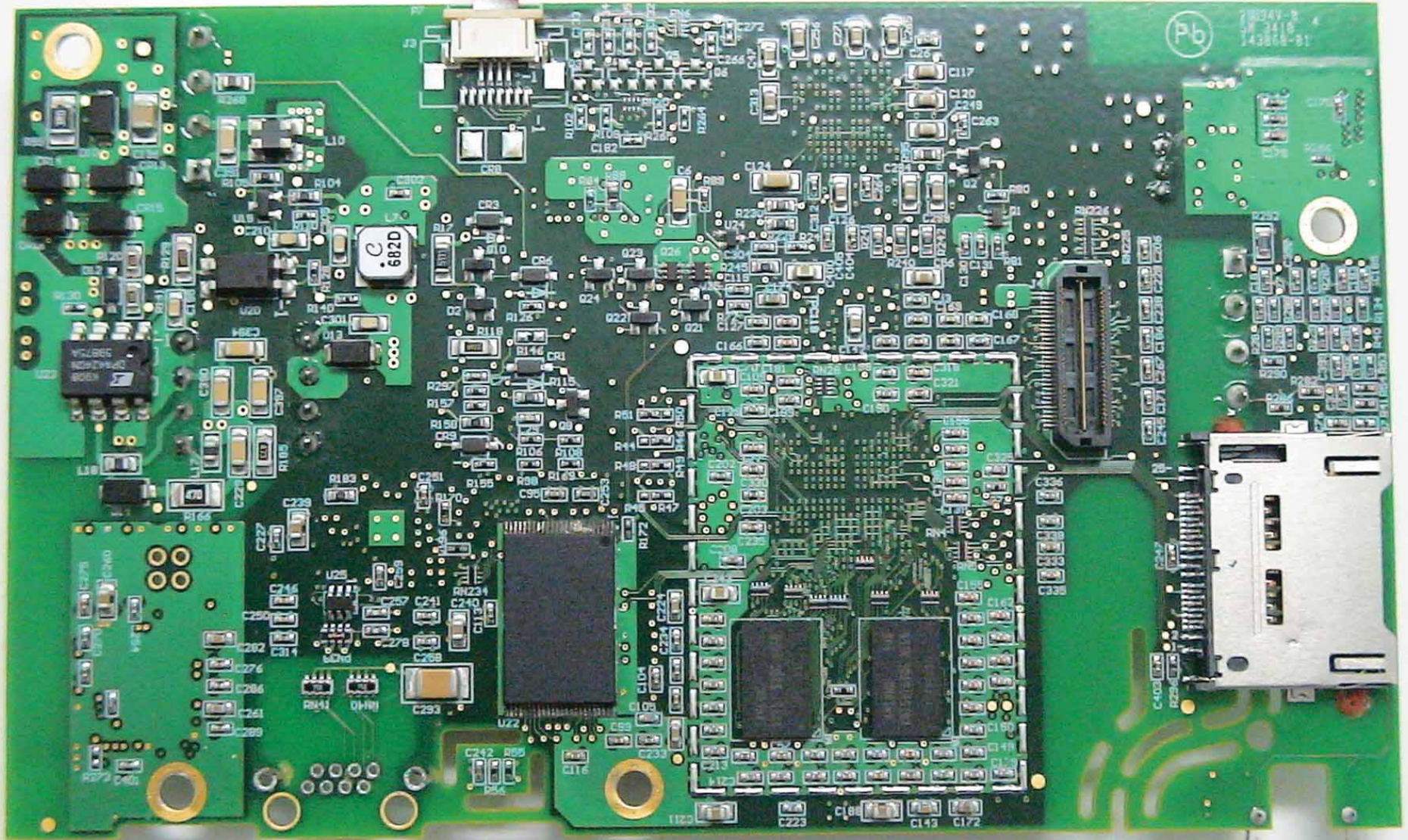
PCB (bottom)
