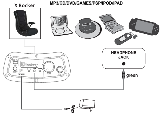
DIAGRAM 3 PORTABLE DEVICES
